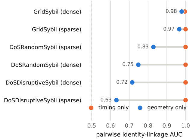
Fig. 3. Timing evidence versus geometric evidence, per archive. Each pair shows one archive under two feature sets. Timing alone sits at or near AUC 1.000 everywhere. Geometry, the physically motivated signal, varies widely. The dashed rule marks chance at AUC 0.5. DataReplaySybil is absent: it yields no concurrent pairs.
