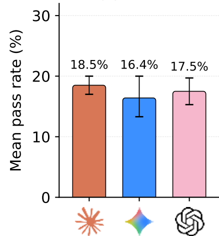
(a) Planner
