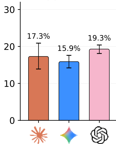
(c) Verifier
