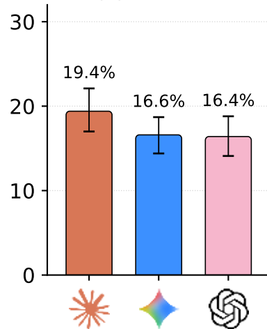
(b) Executor
