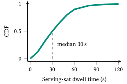
Fig. 2. Serving-satellite dwell-time CDF; median 30 s.
