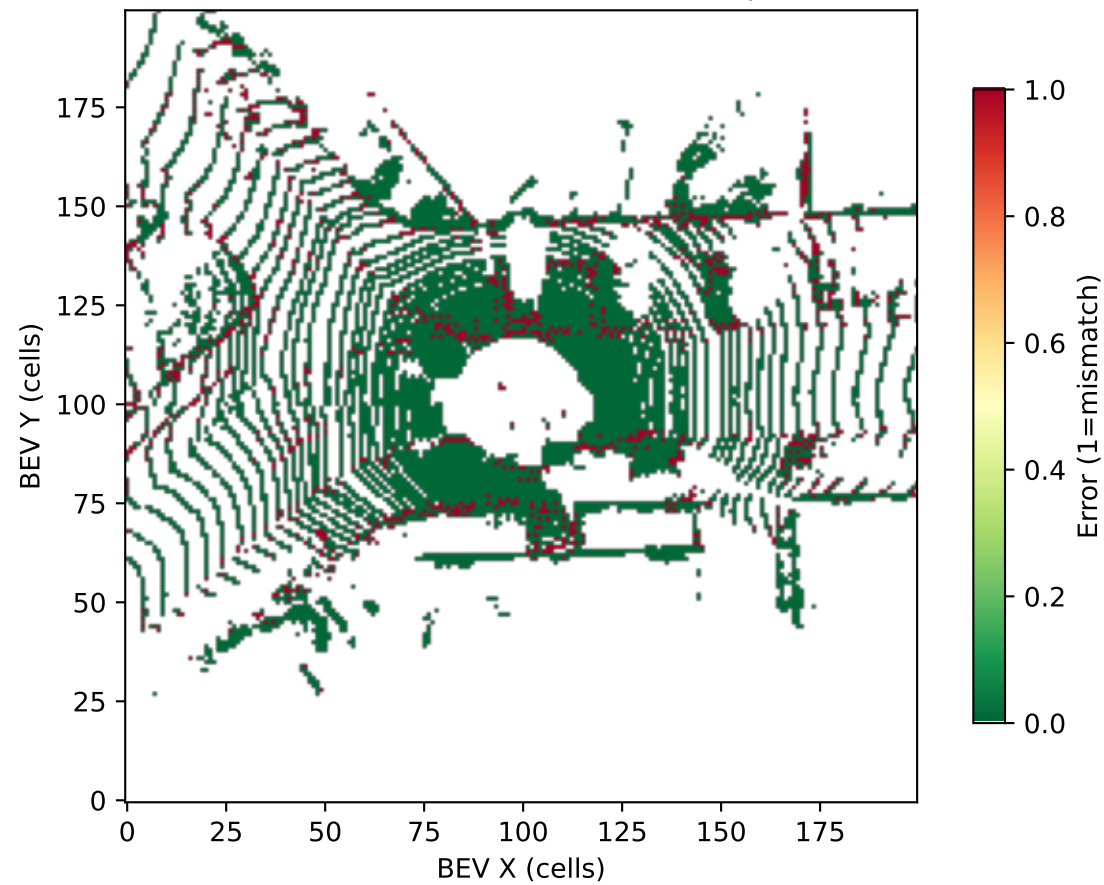
(c) BEV Reconstruction Error Map
