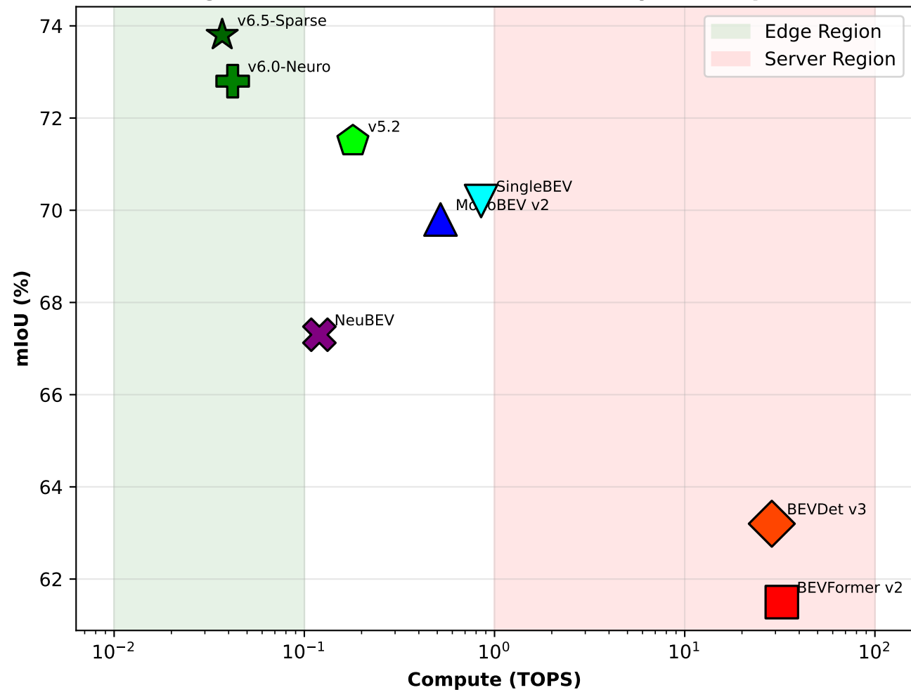
Figure 4a: Pareto Frontier ? Accuracy vs Compute
