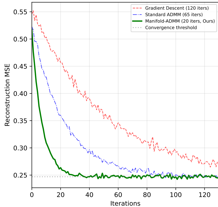
(a) Optimizer Convergence Curves
