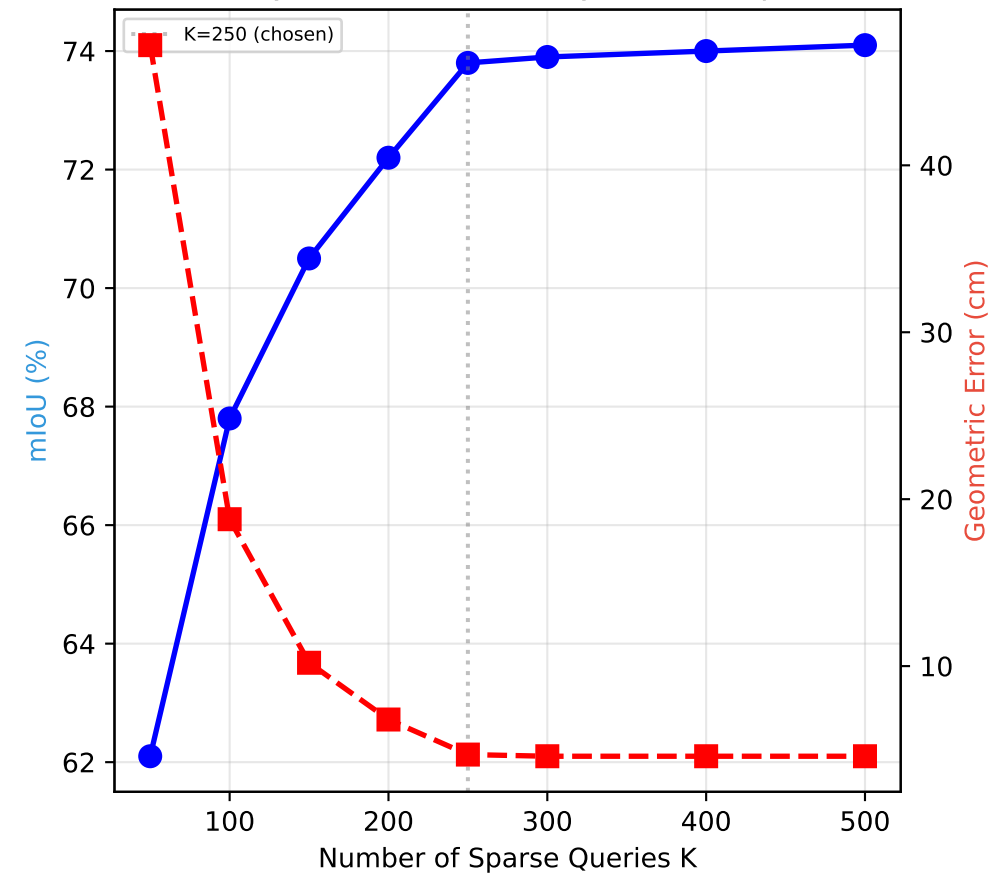
(c) Query Count vs Accuracy (K=250 optimal)
