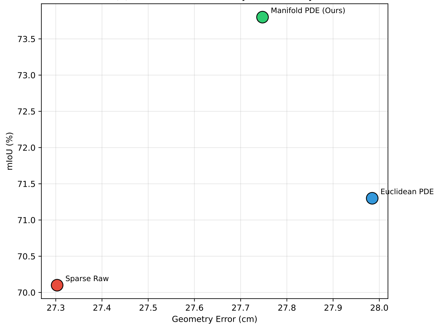
(c) Query Strategy Comparison
