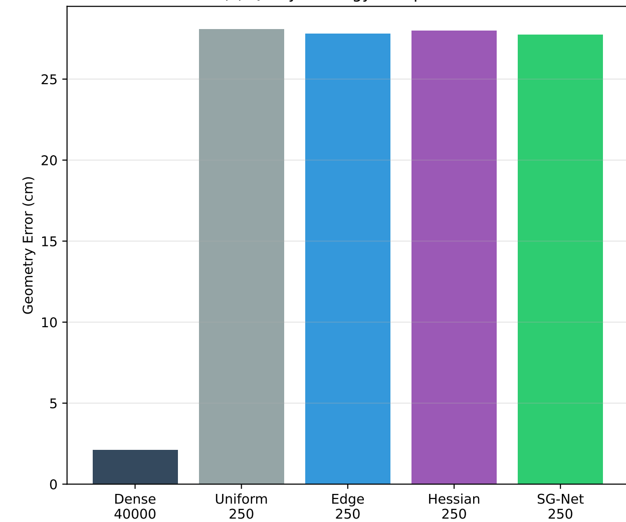
(c) Query Strategy Comparison
