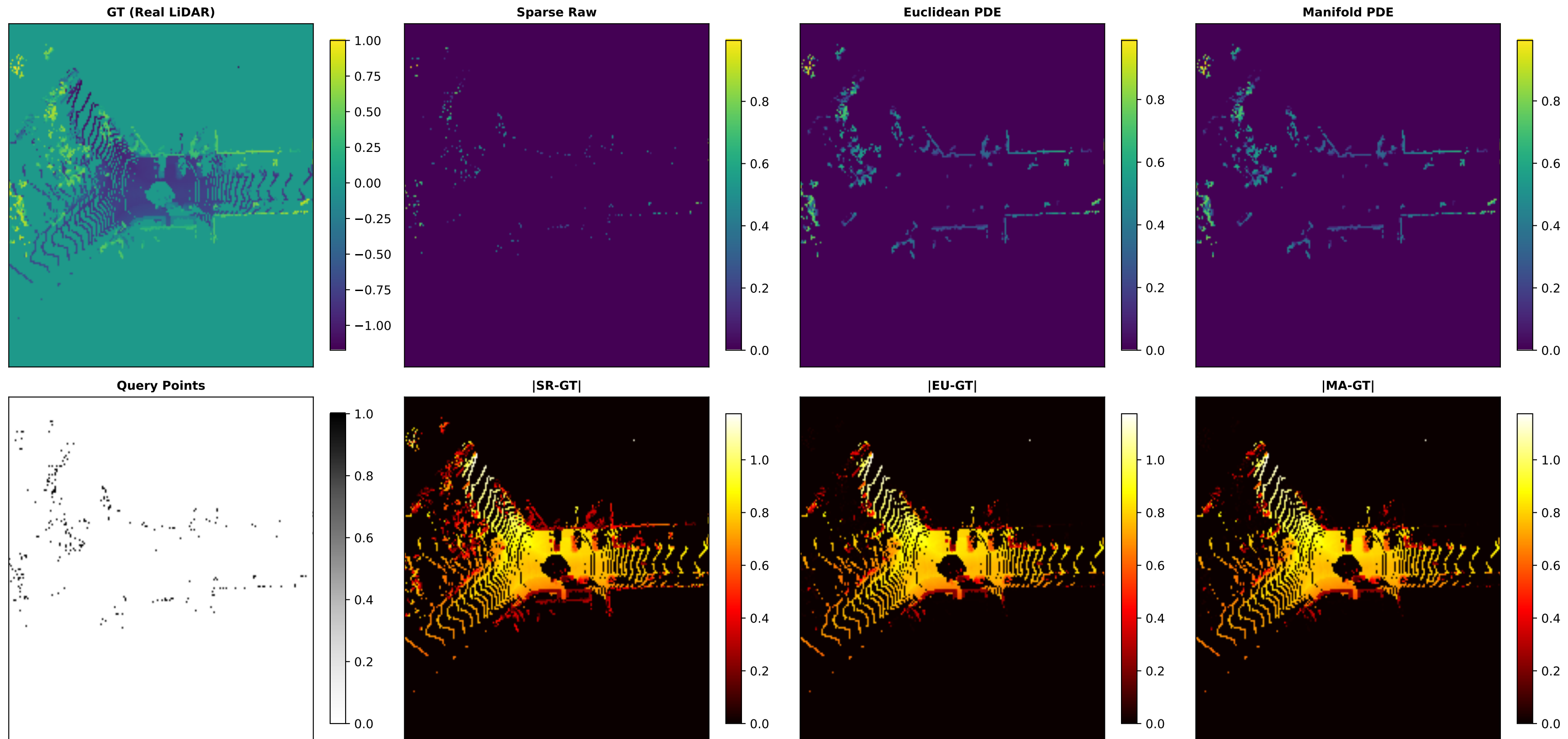
FIG 4b: Visual Comparison — SE_000008 (SemanticKITTI, 64ch_HDL64E)
