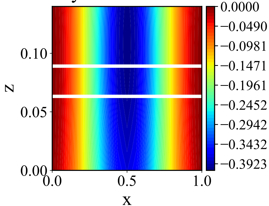
Three-Layer FEA Cross-Section
