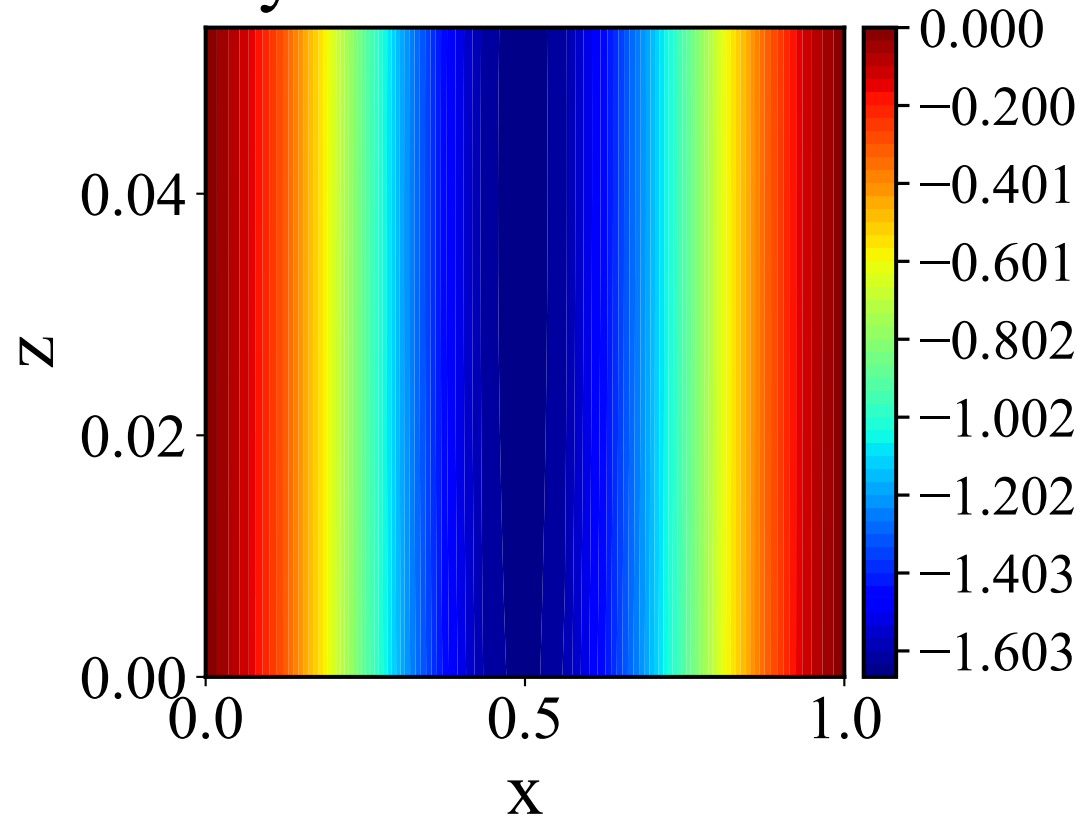
One-Layer PINN Cross-Section
