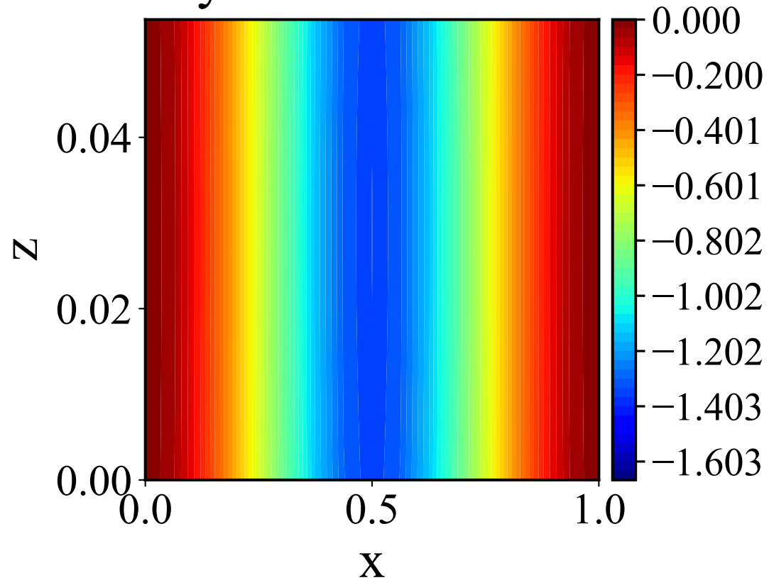
One-Layer FEA Cross-Section
