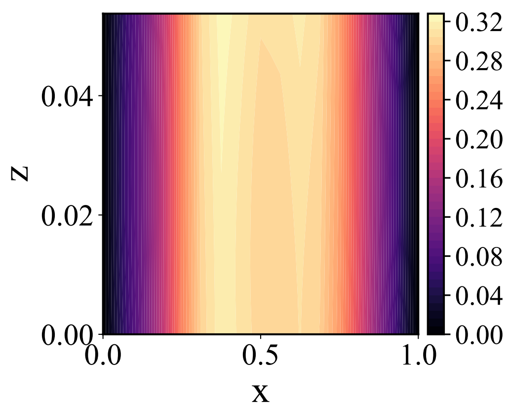
Abs Error Cross-Section Volume MAE=2.87%
