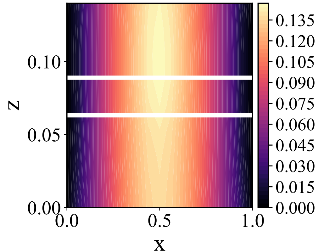
Abs Error Cross-Section Volume MAE=4.66%
