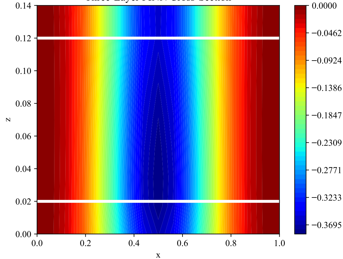
Three-Layer PINN Cross-Section
