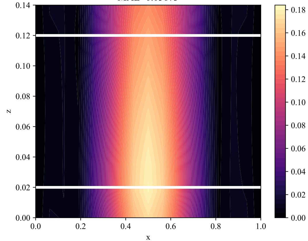
Abs Error Cross-Section MAE=0.05673
