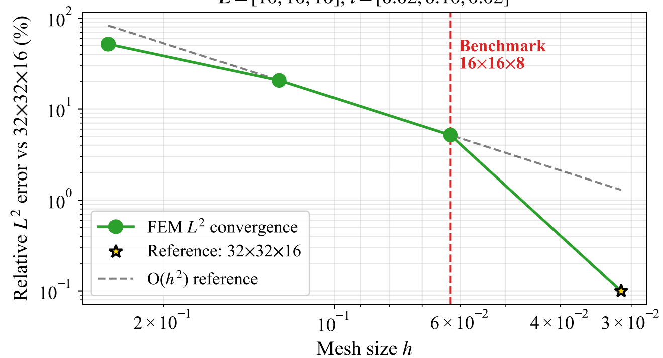
(d) Three-Layer: L^2 Convergence Rate E = [10, 10, 10], t = [0.02, 0.10, 0.02]
