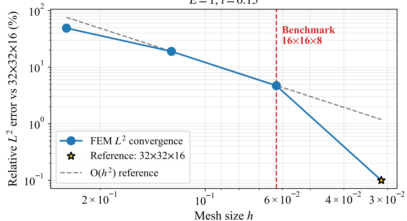
(b) One-Layer: L^2 Convergence Rate E = 1, t = 0.15
