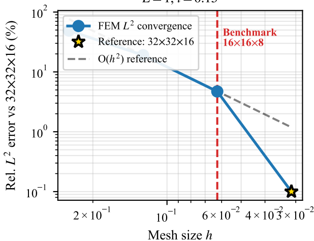
(b) L^2 Convergence Rate E = 1, t = 0.15
