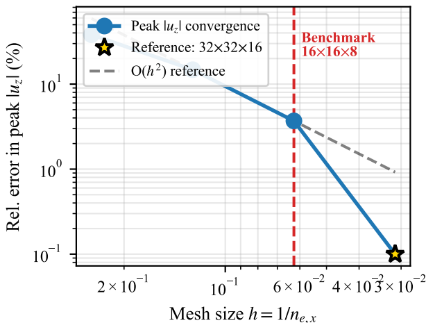
(a) Peak Displacement Convergence E = 1, t = 0.15
