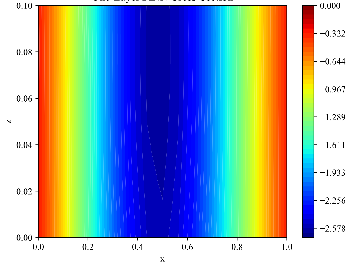
One-Layer PINN Cross-Section
