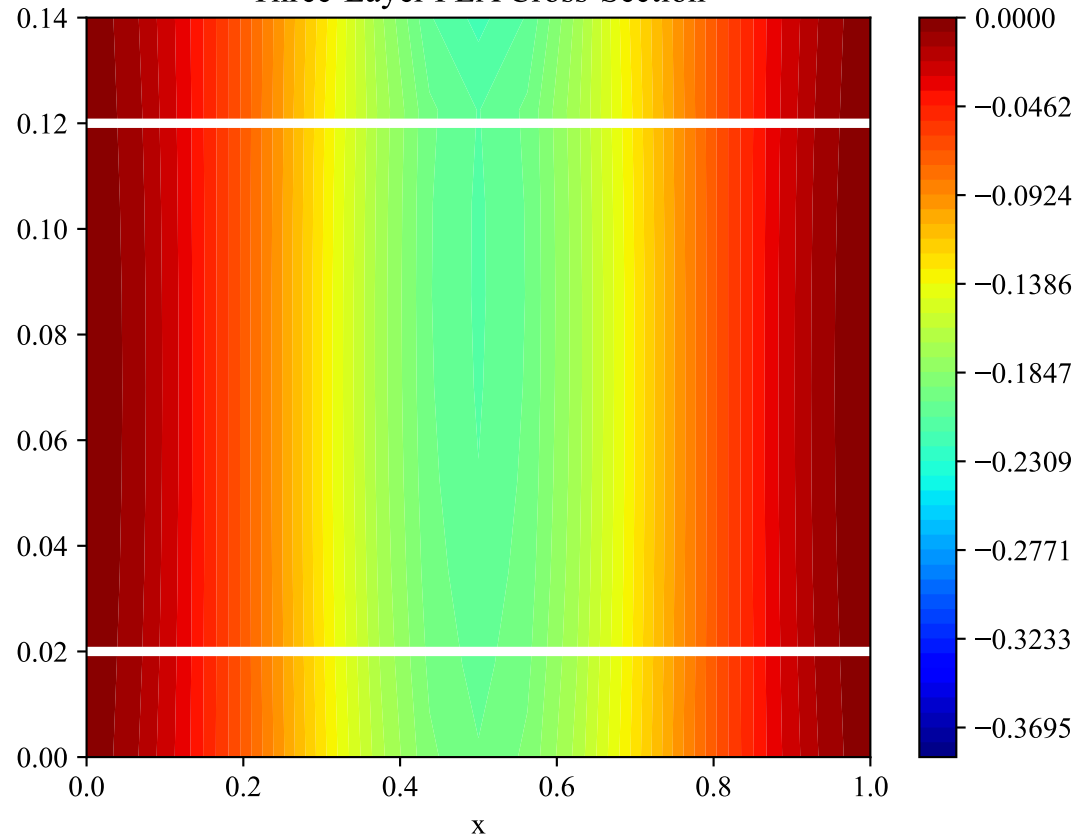
Three-Layer FEA Cross-Section
