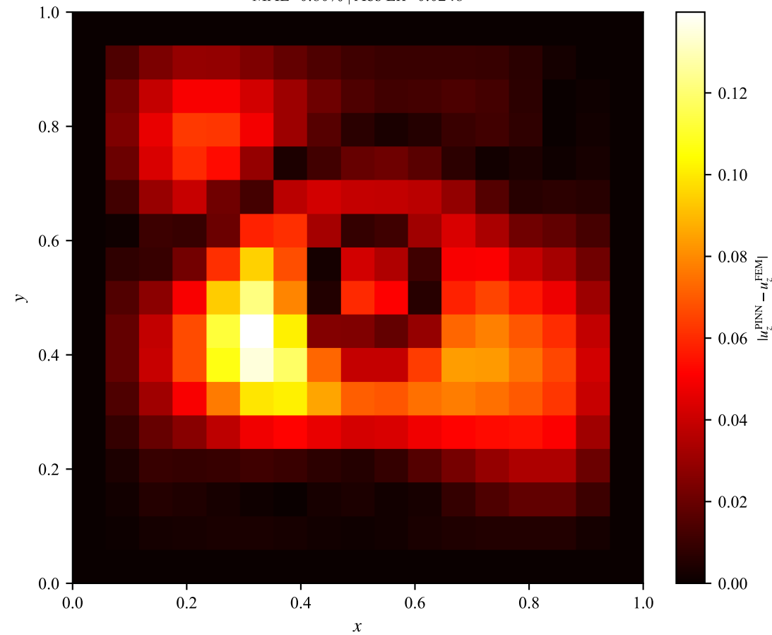
(a) One-Layer: Best Case E = 1.36, t = 0.083 MAE=0.80% | Abs Err=0.0248
