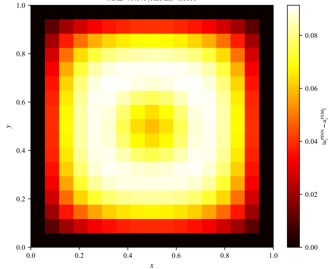
(c) Three-Layer: Best Case E = [1.3, 7.5, 6.9] t = [0.029, 0.031, 0.100] MAE=7.48% | Abs Err=0.0116
