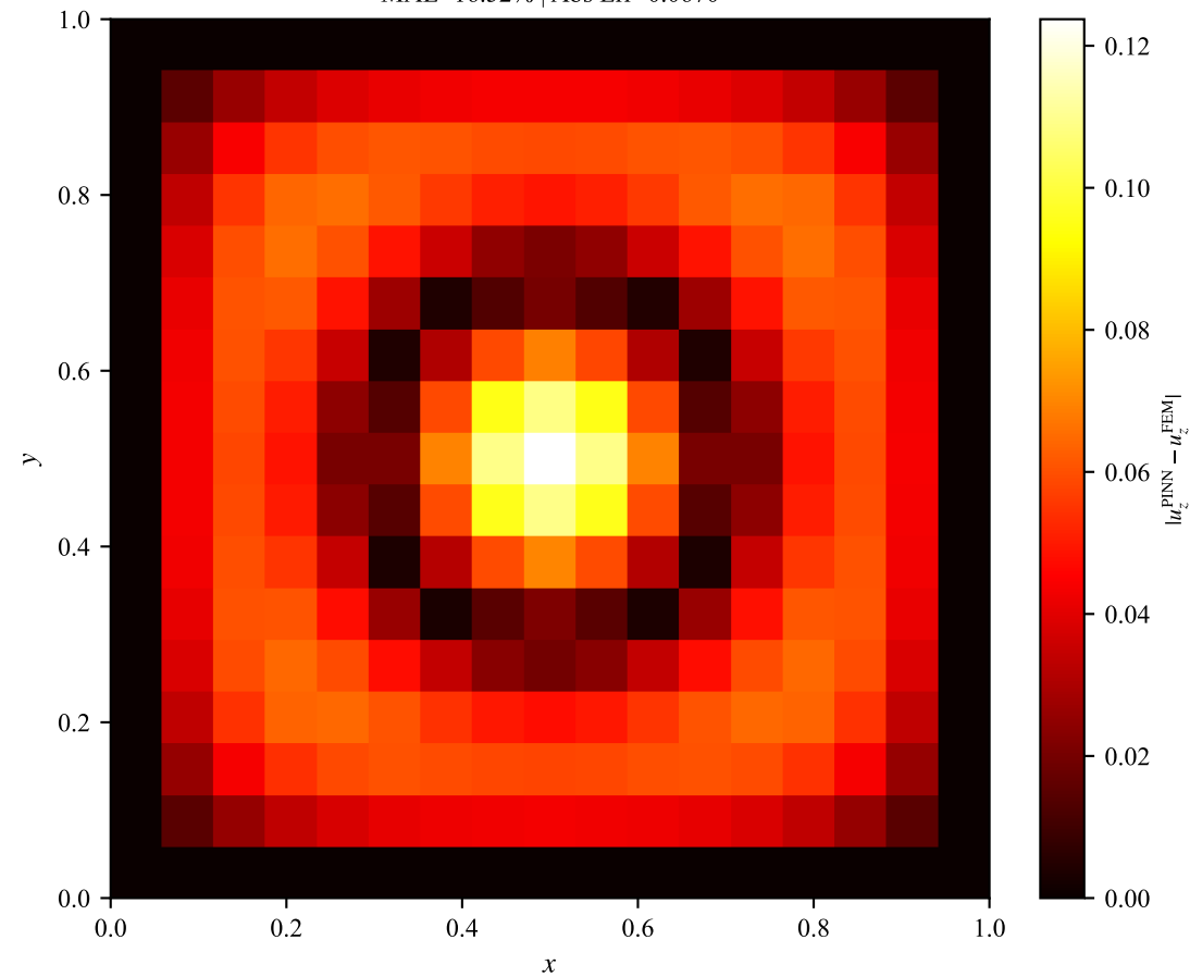
(d) Three-Layer: Worst Case E = [1.2, 9.3, 7.2] t = [0.063, 0.026, 0.051] MAE=16.52% | Abs Err=0.0670
