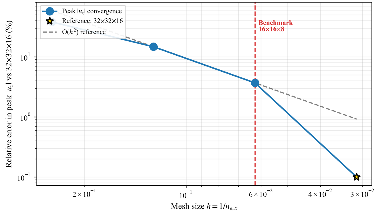
(a) One-Layer: Peak Displacement Convergence E = 1, t = 0.15
