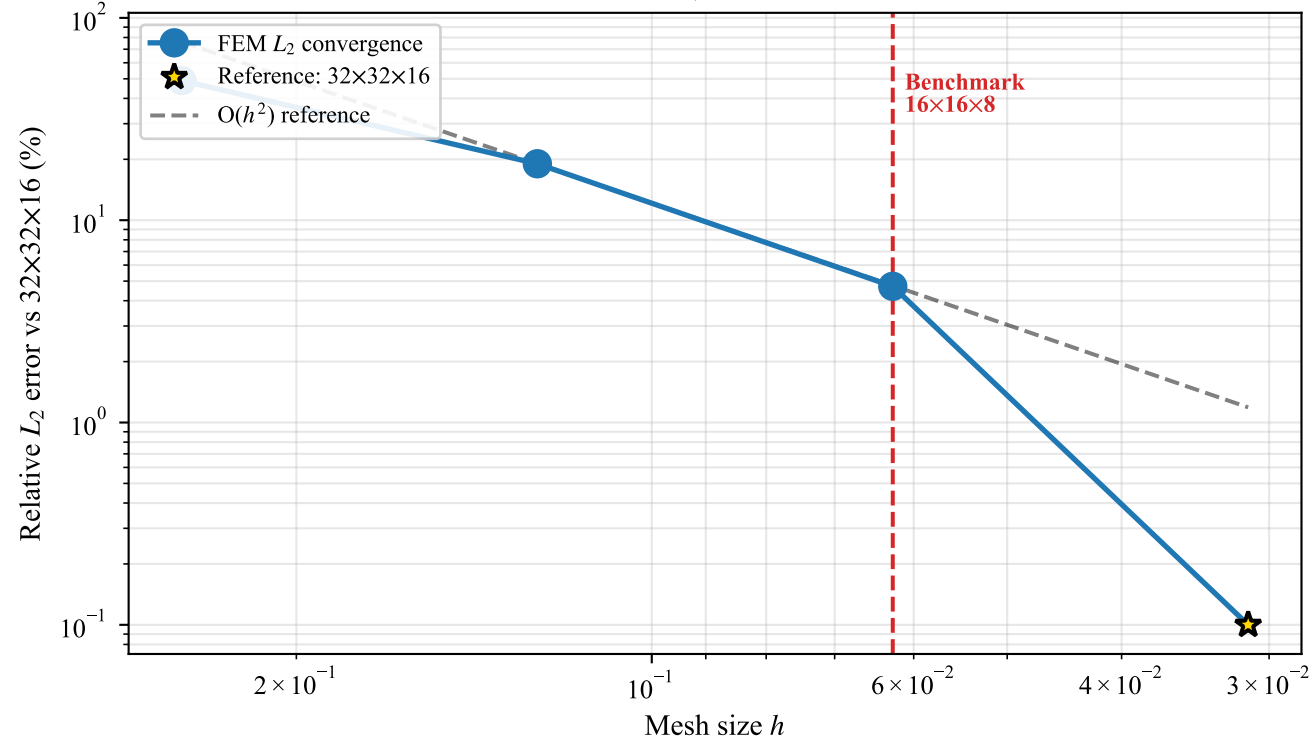
(b) One-Layer: L_2 Convergence Rate E = 1, t = 0.15
