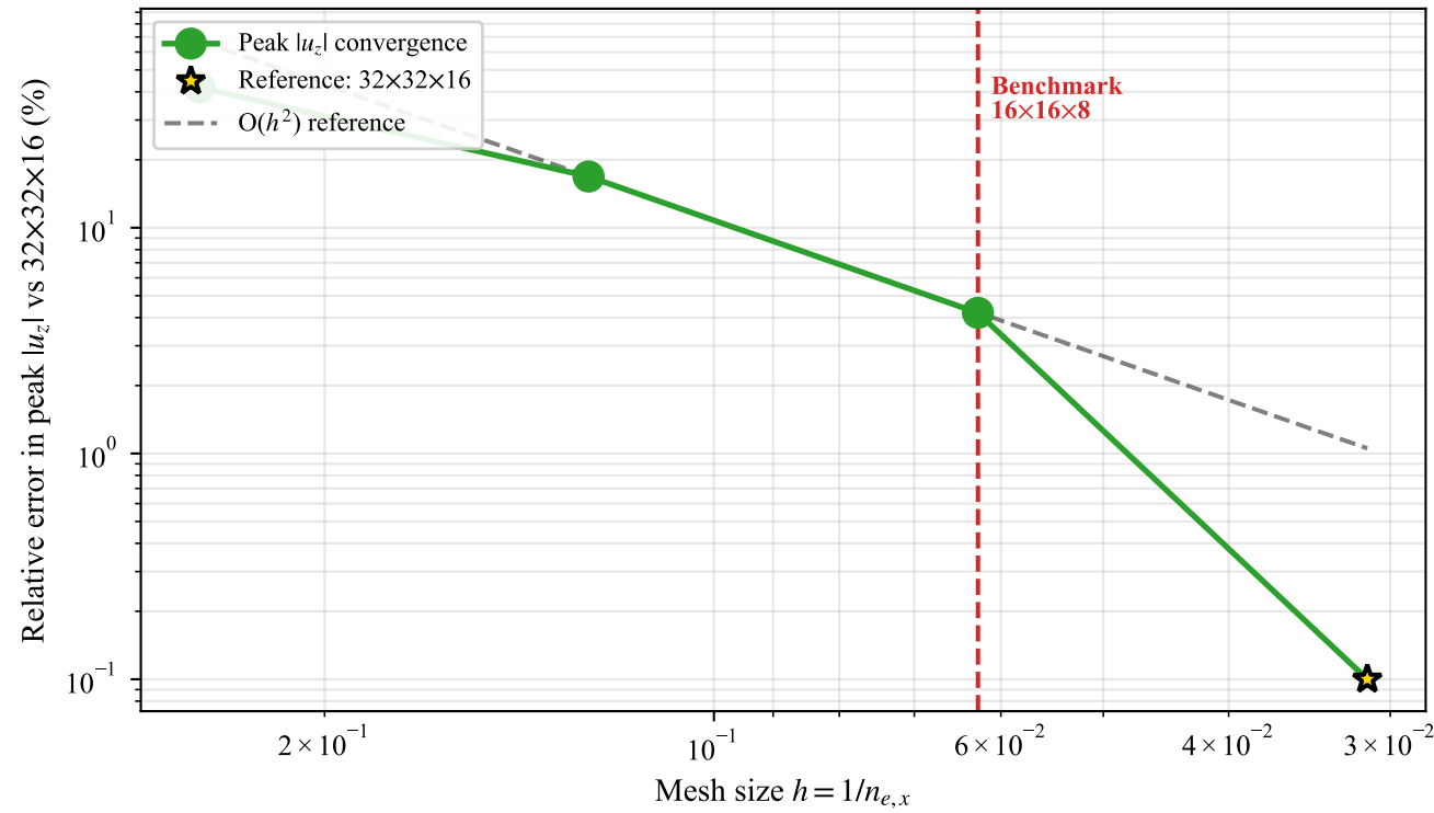
(c) Three-Layer: Peak Displacement Convergence E = [10, 10, 10], t = [0.02, 0.10, 0.02]
