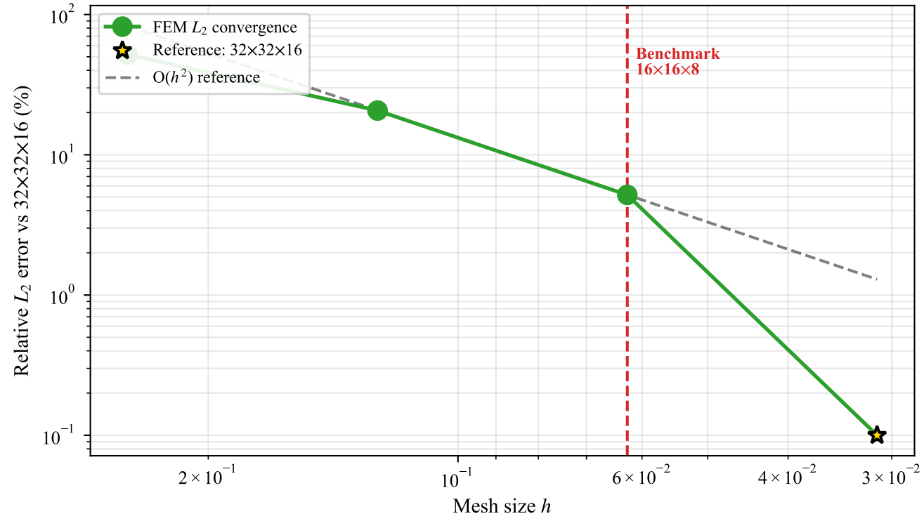
(d) Three-Layer: L_2 Convergence Rate E = [10, 10, 10], t = [0.02, 0.10, 0.02]
