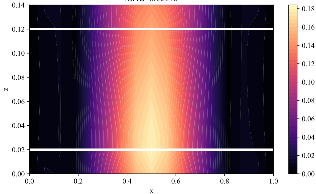
Abs Error Cross-Section MAE=0.05673
