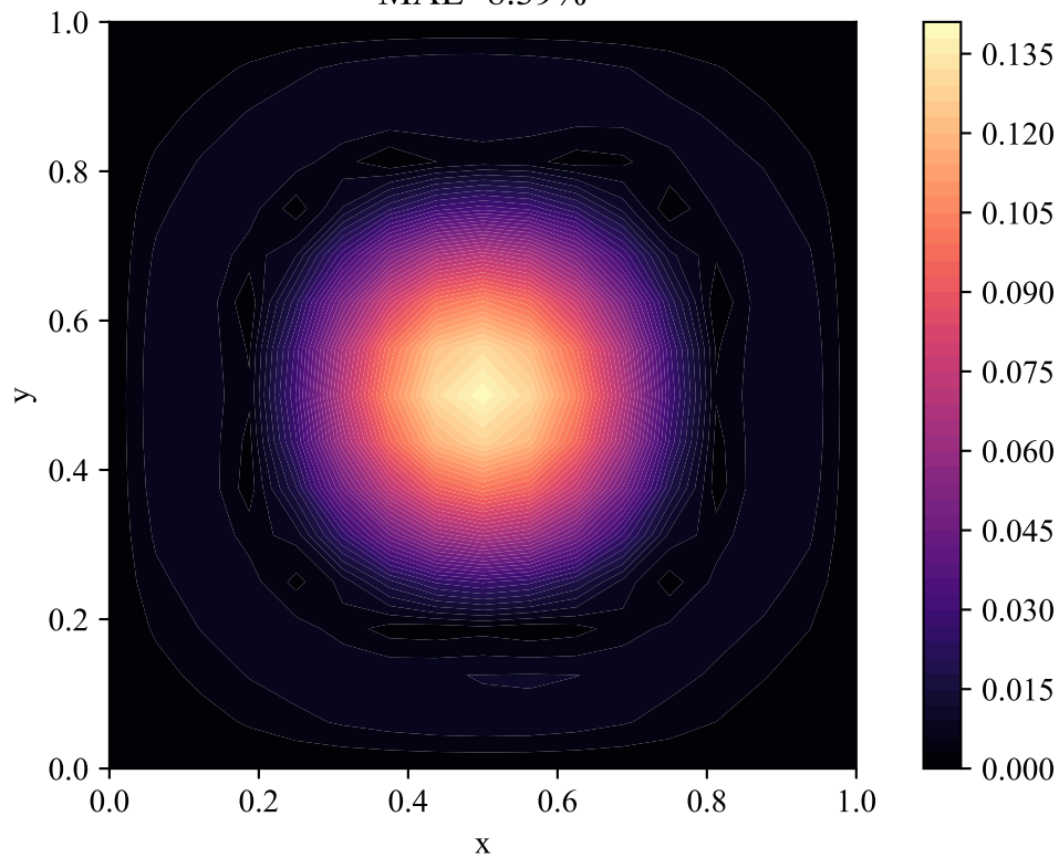
Abs Error MAE=8.39%
