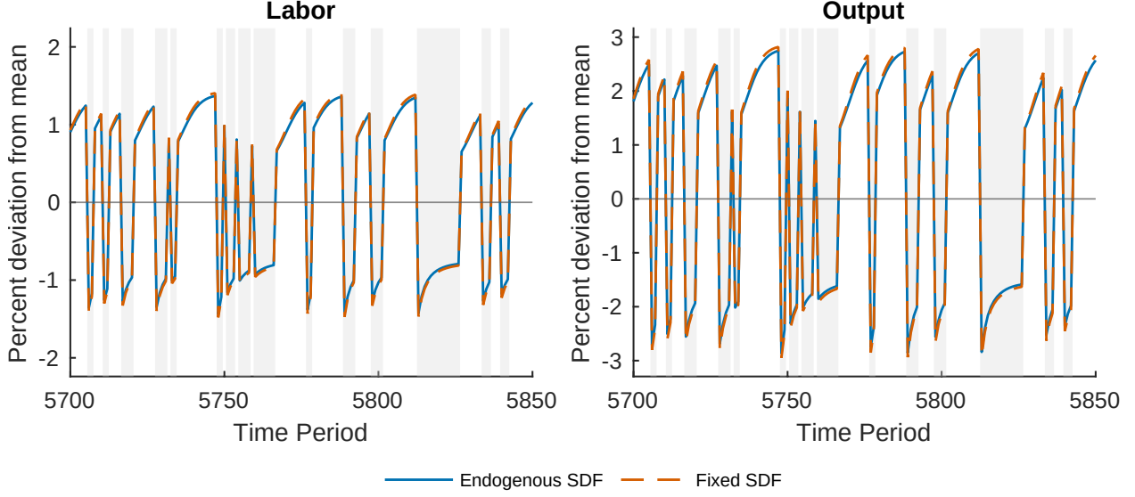
Figure C.2: Benchmark and fixed-SDF counterfactual
