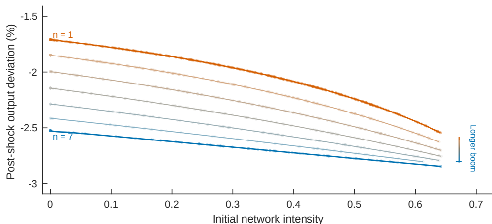
Figure C.1: Joint size and duration dependence in output shock responses
