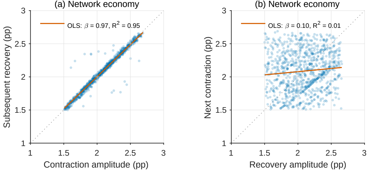
Figure D.4: Predictability asymmetry in the model-implied plucking component
