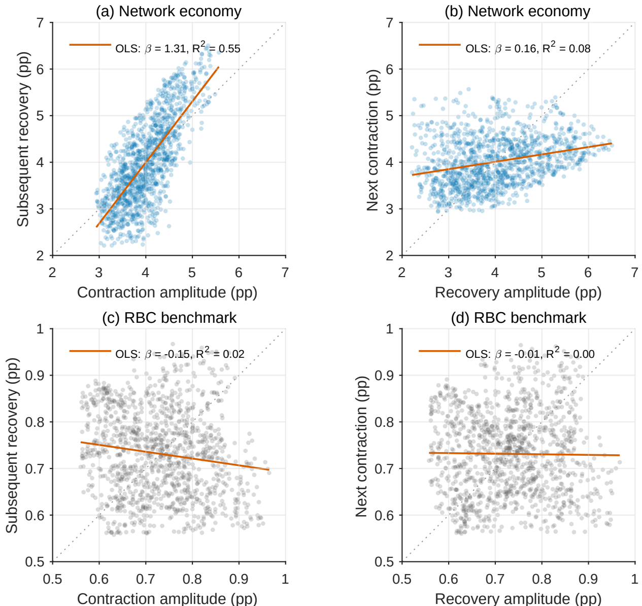
Figure D.3: Plucking-cycle exercise for simulated output slack
