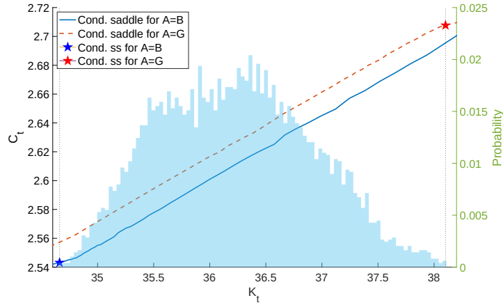
Figure 5: Conditional saddle paths in Krusell and Smith (1998)
