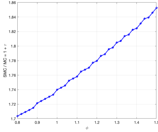
(c) Proportional wedge SMC/MC = 1 + \tau
