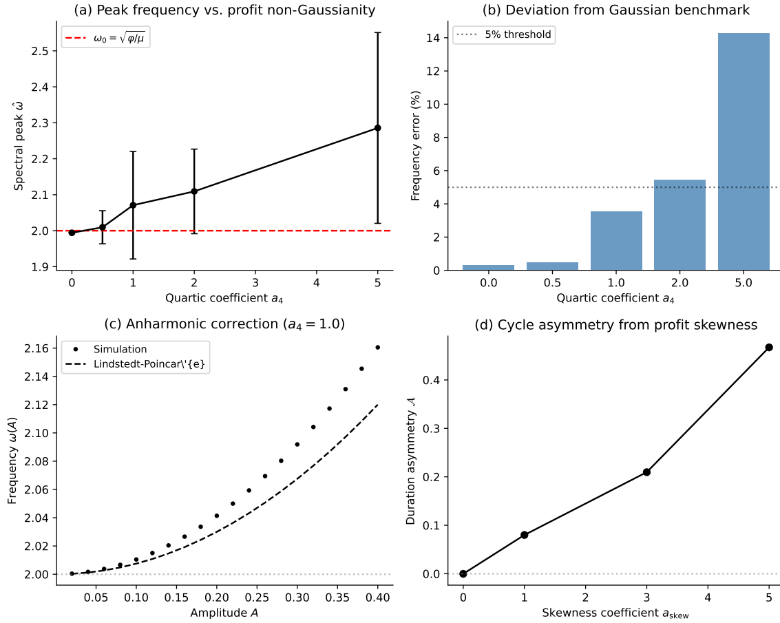
Figure C.5: log-quadratic approximation error under quartic and skewed profit perturbations
