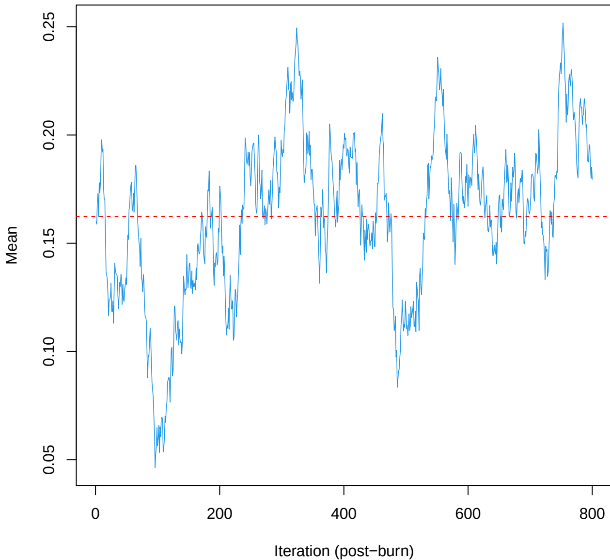
SCE3 | k=4 | \mu[\text{comp3, PC7}]
