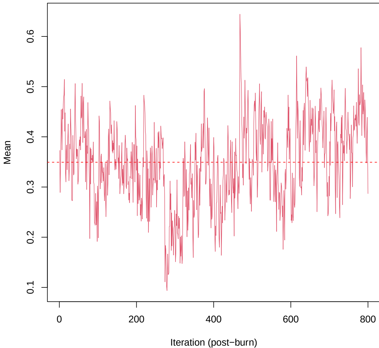
SCE2 | k=3 | mu[comp1, hars_score]
