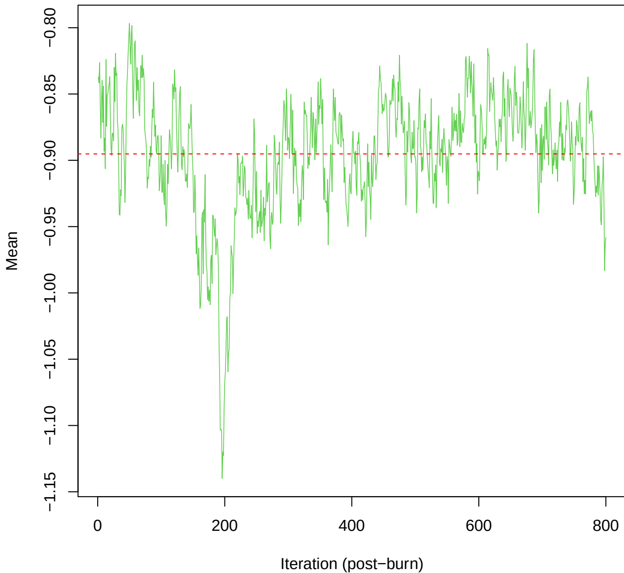
SCE2 | k=4 | \mu[\text{comp2}, \text{hars\_score}]
