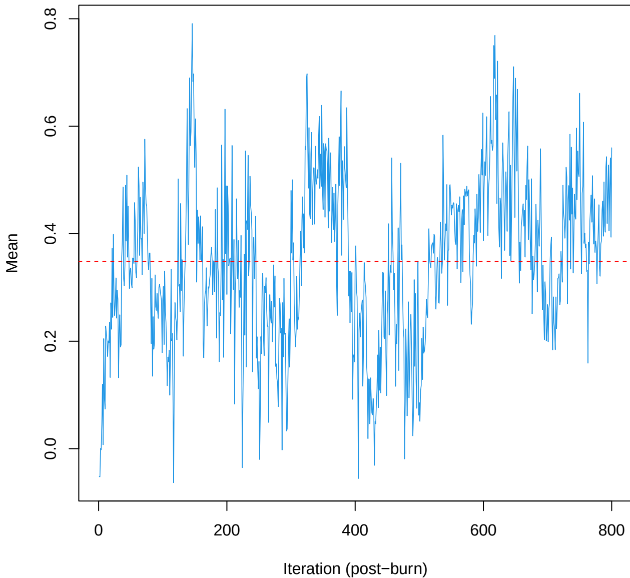
SCE2 | k=4 | \mu[\text{comp3}, \text{hars\_score}]
