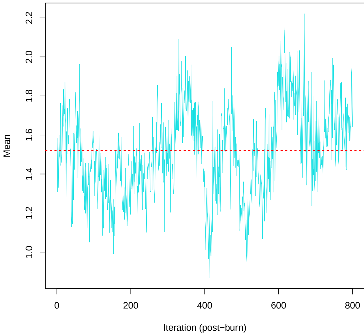
SCE2 | k=4 | mu[comp4, hars_score]
