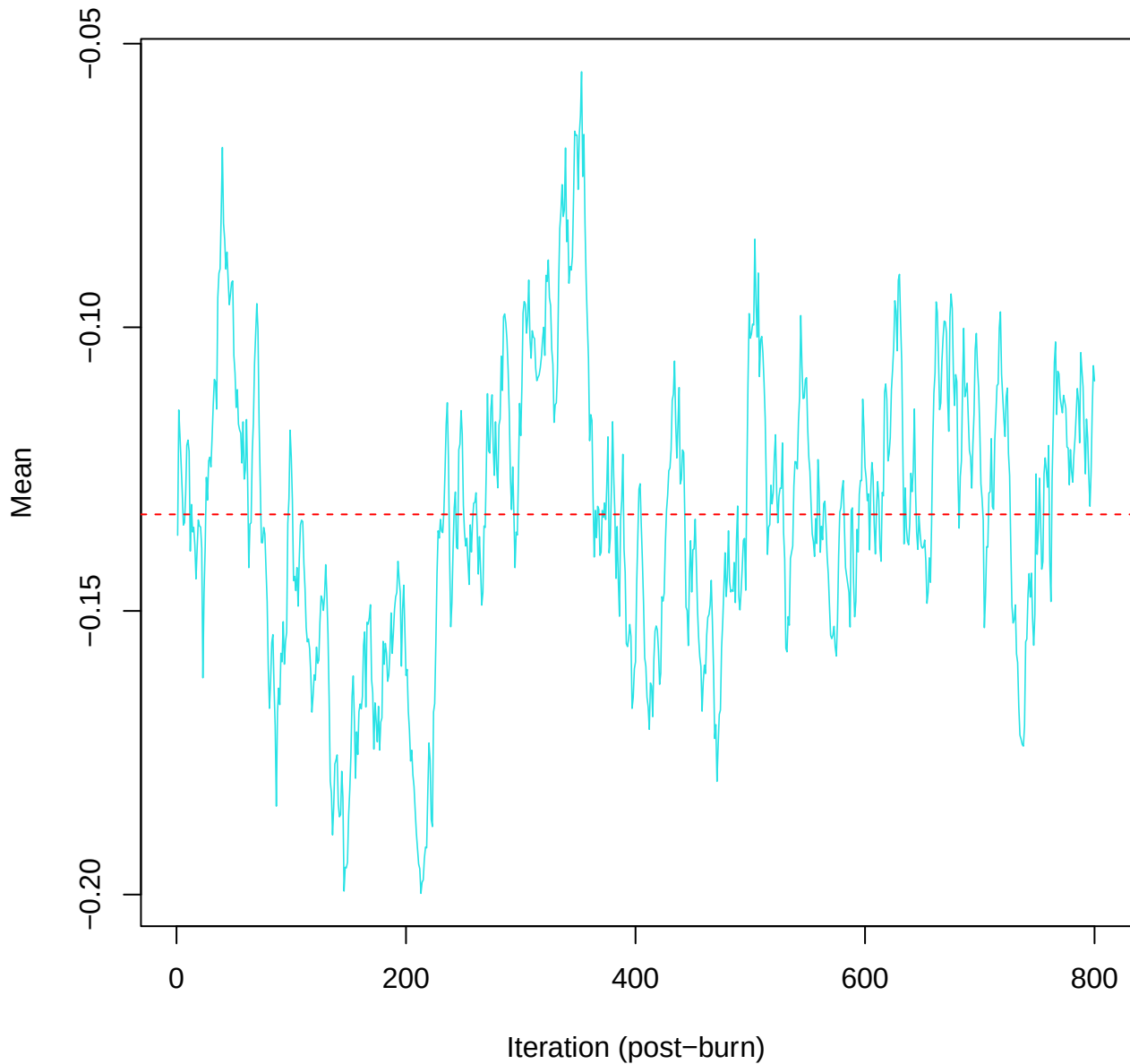
SCE3 | k=5 | \mu[\text{comp4}, \text{PC7}]
