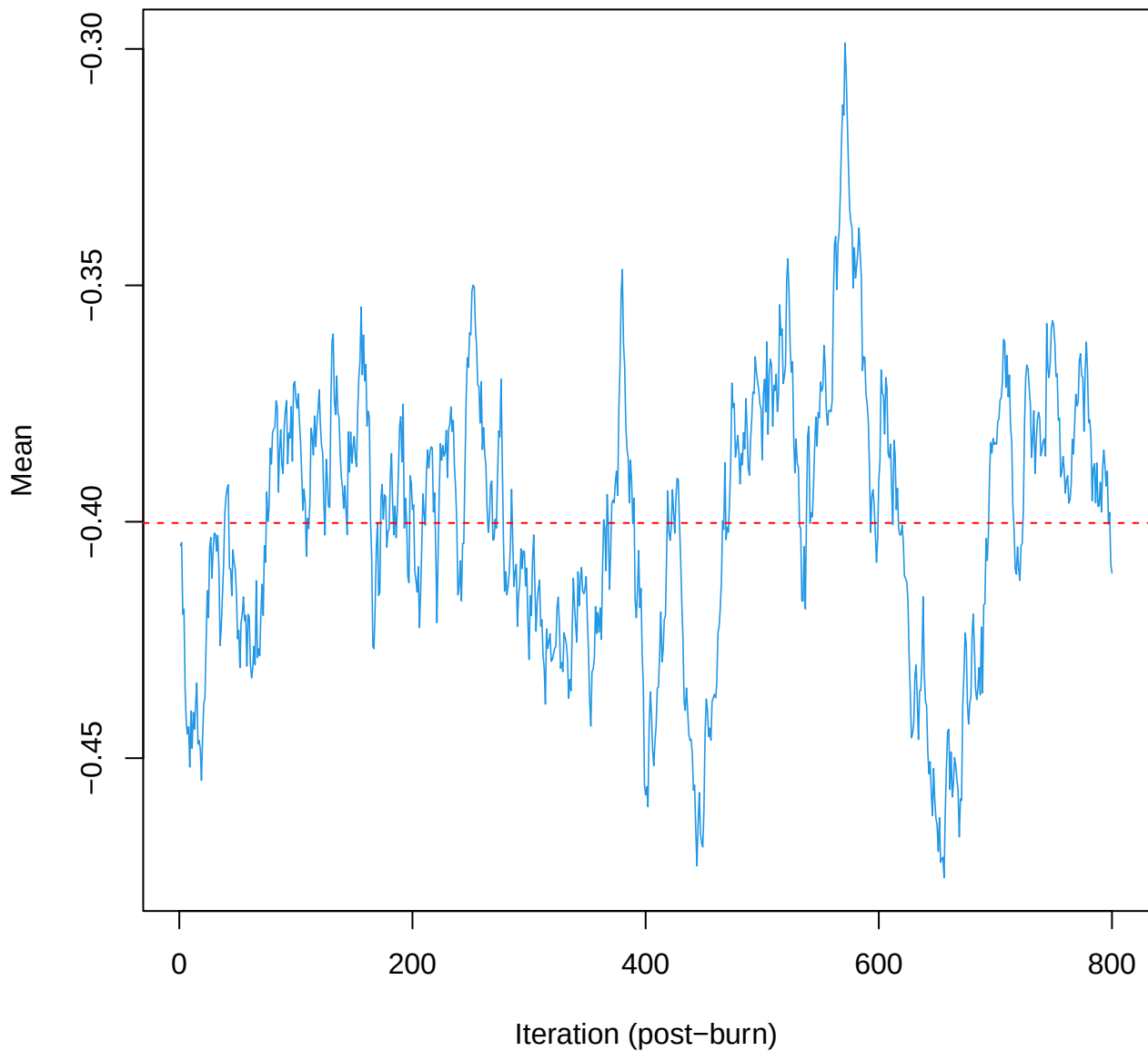
SCE3 | k=4 | \mu[\text{comp3, PC1}]
