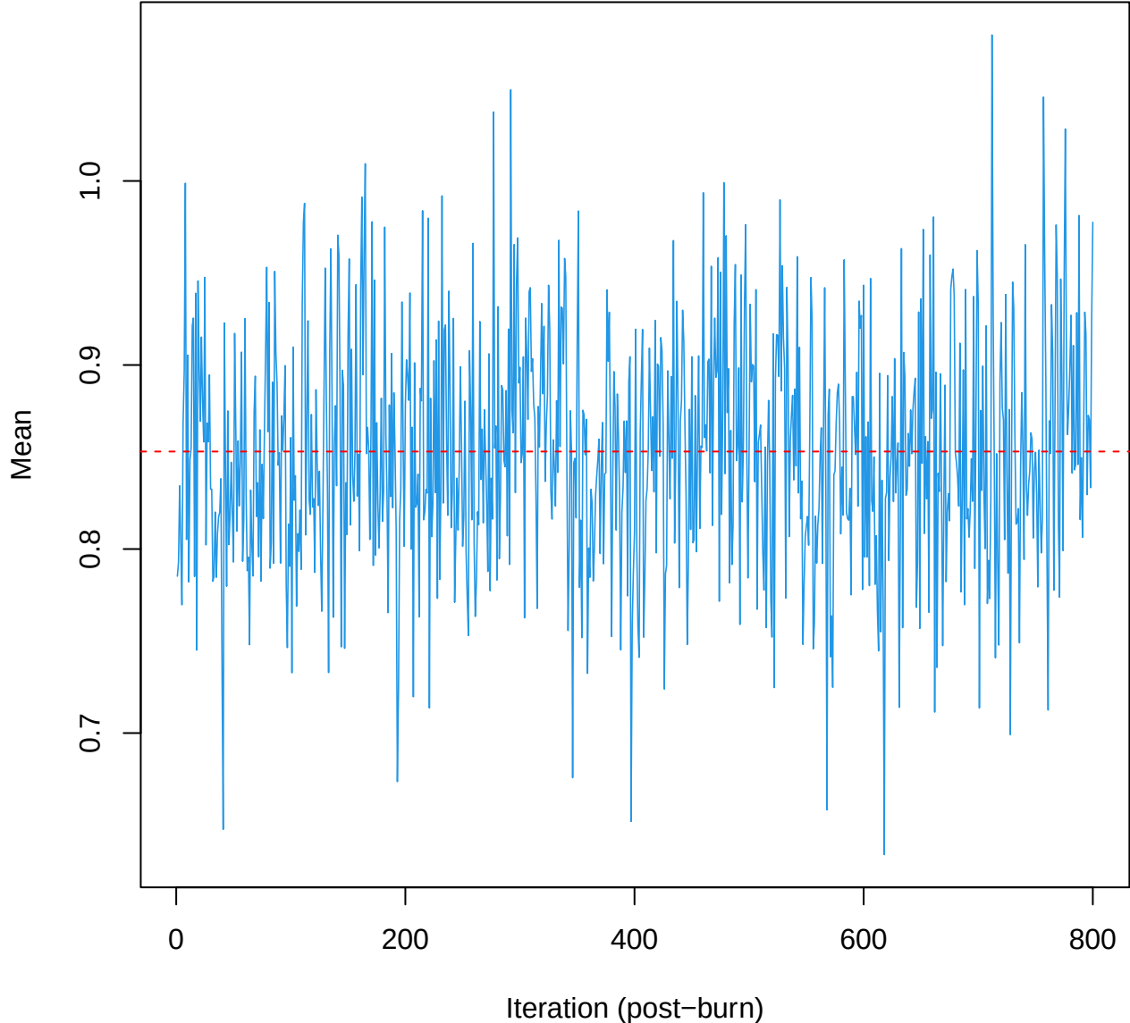
SCE3 | k=3 | mu[comp3, PC1]
