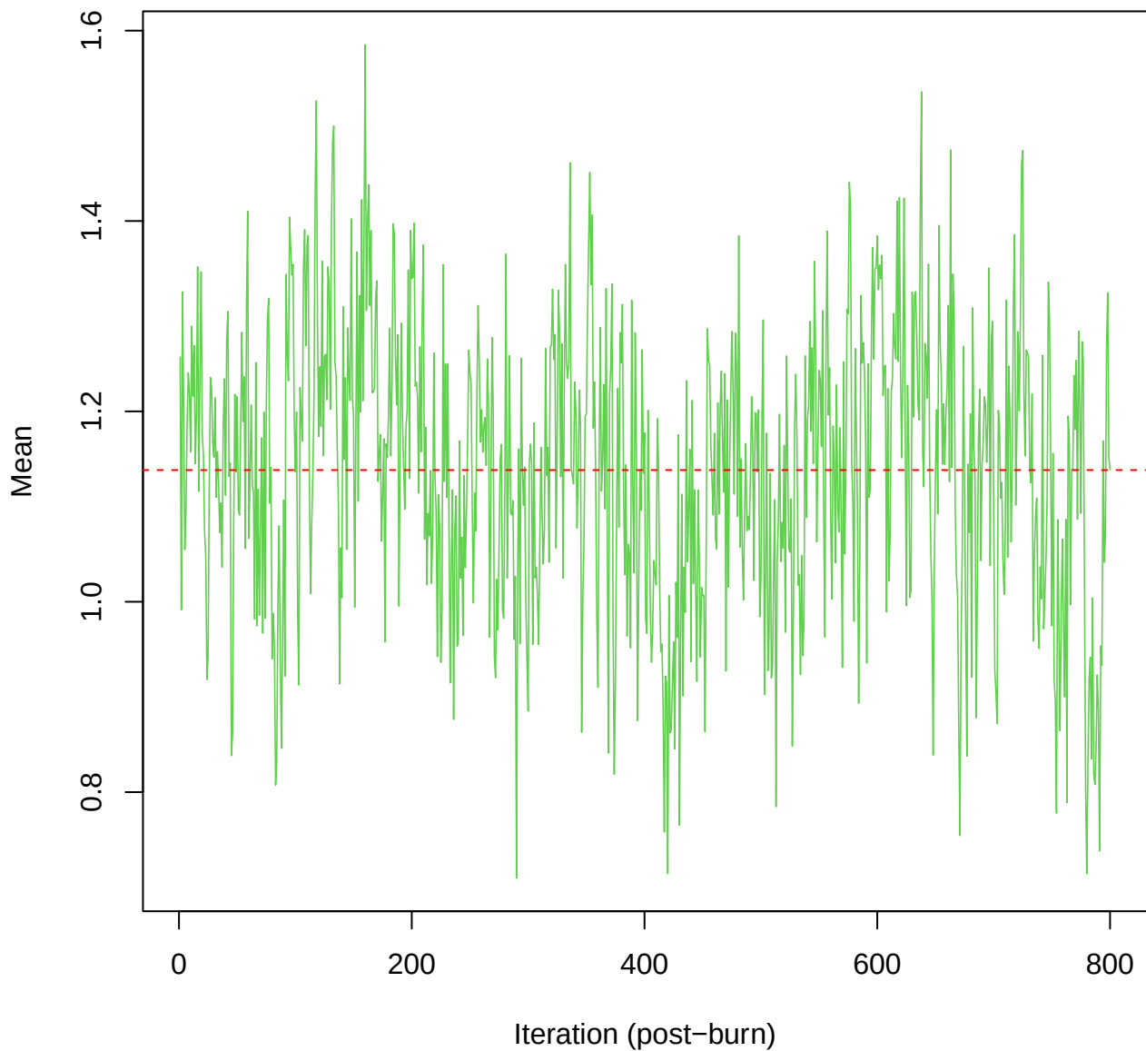
SCE2 | k=2 | \mu[\text{comp2}, \text{hars\_score}]
