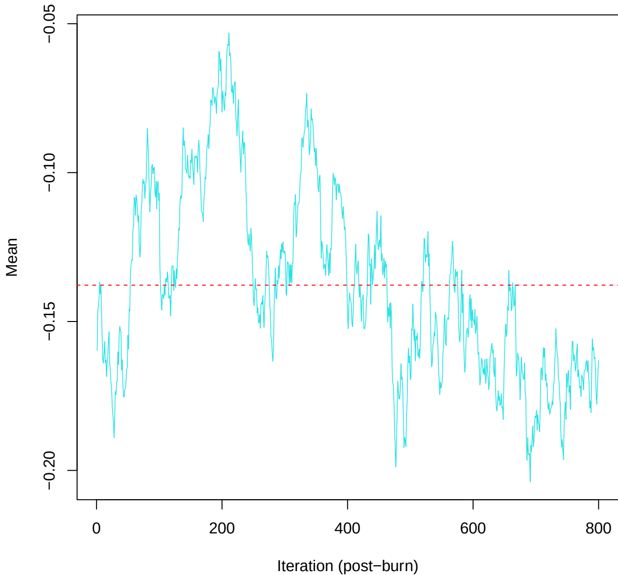
SCE3 | k=5 | \mu[\text{comp4}, \text{PC4}]
