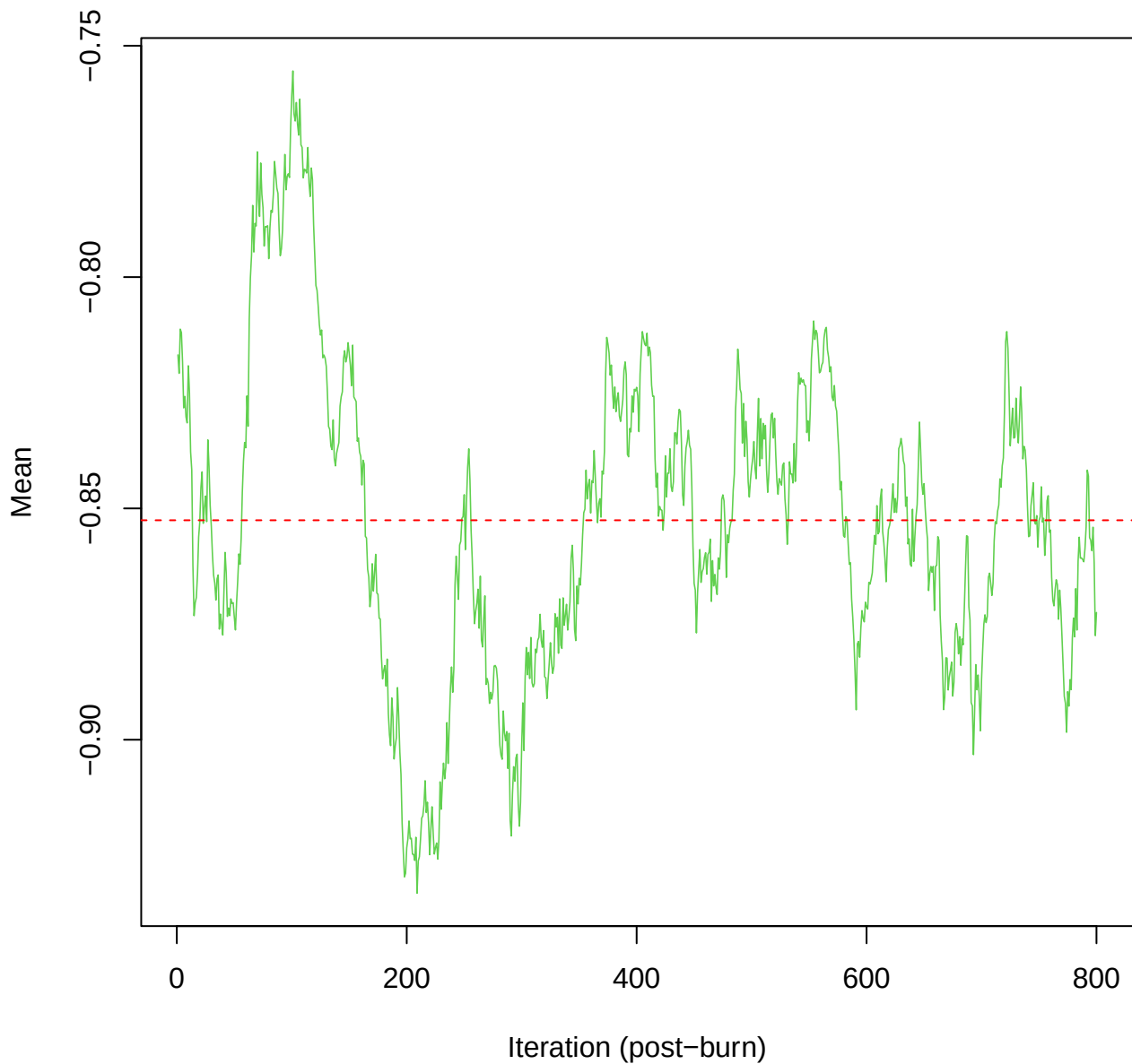
SCE3 | k=4 | mu[comp2, PC1]
