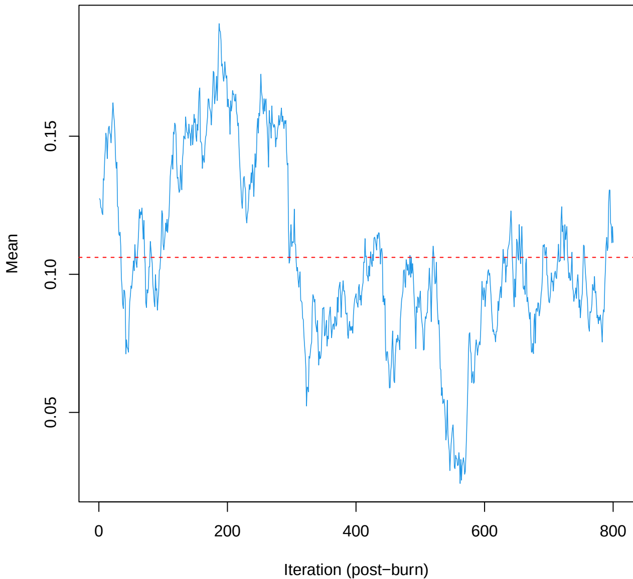
SCE3 | k=5 | mu[comp3, PC6]
