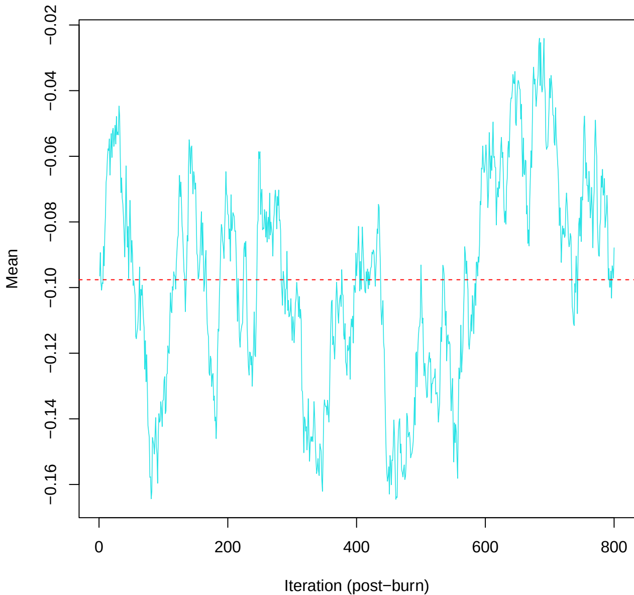
SCE3 | k=4 | \mu[\text{comp4}, \text{PC5}]
