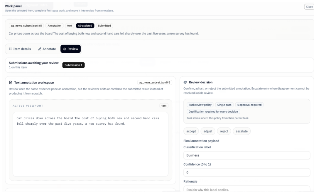
Figure 2. A reviewer judging the AI's first pass (Llama 3 labelled this headline "Business")
