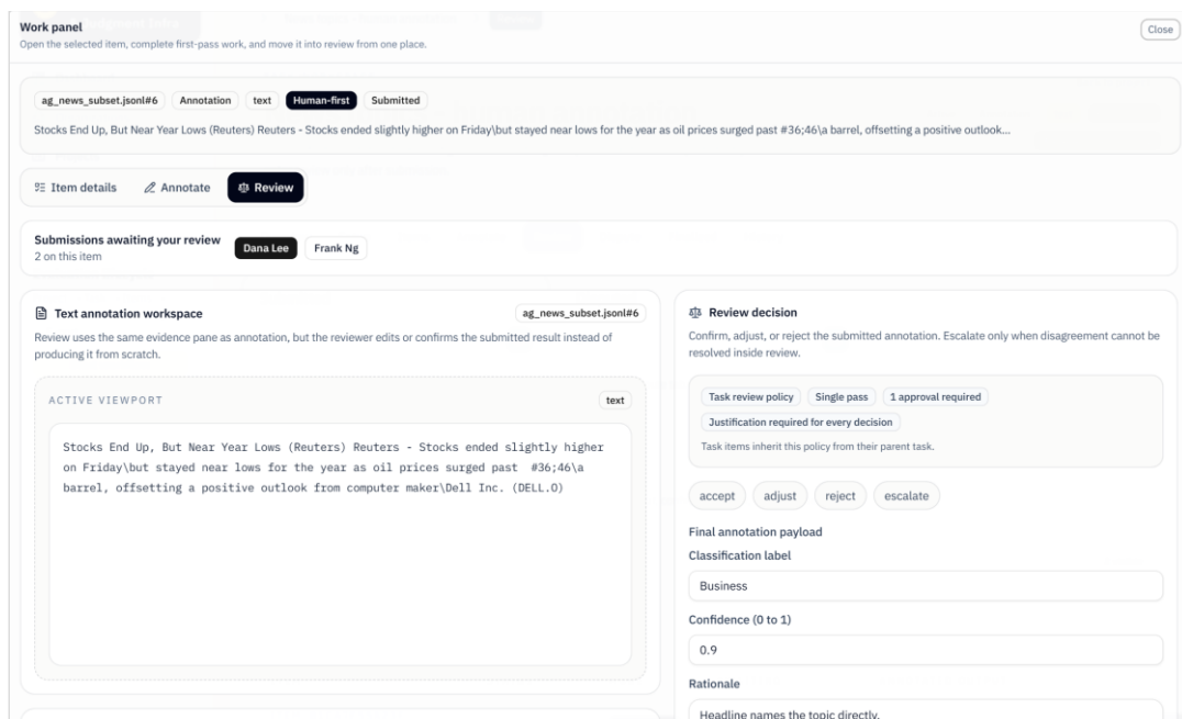
Figure 3. The review panel: two submissions await review on this item, and the reviewer picks one
