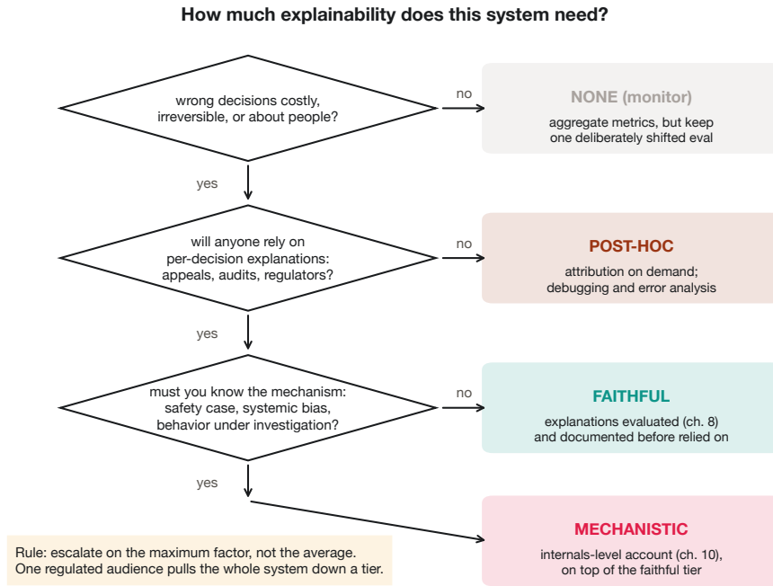
Figure 1.9: Three questions route any system to one of four depths: none, post-hoc, faithful, or mechanistic. The amber rule at the bottom left: escalate on the maximum factor.
