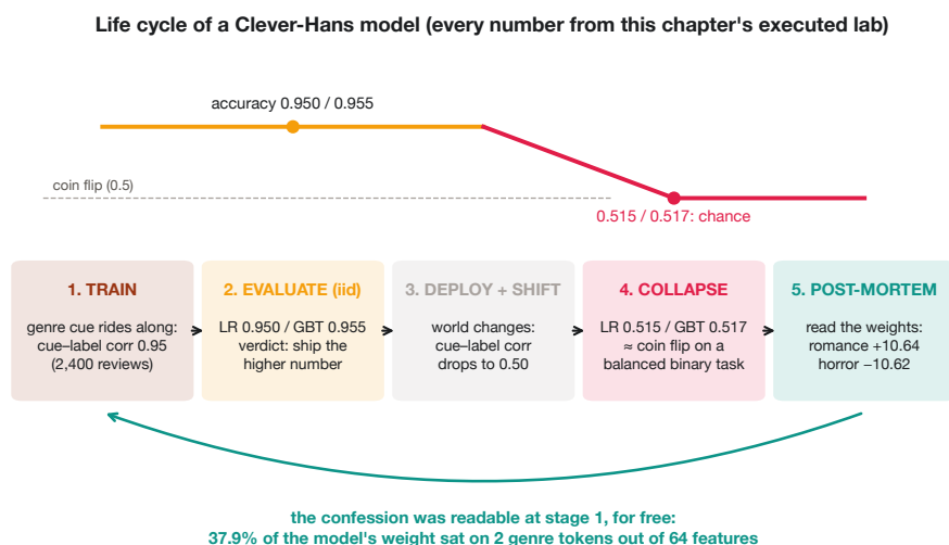
Figure 1.3: The Clever-Hans lifecycle. Accuracy falls from 0.950/0.955 to 0.515/0.517 when the cue decorrelates, and the post-mortem evidence was readable before anything shipped.
