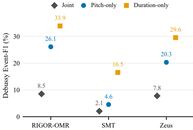
Figure 4: Joint, pitch-only, and duration-only Event-F1 on Debussy for the three frozen methods.
