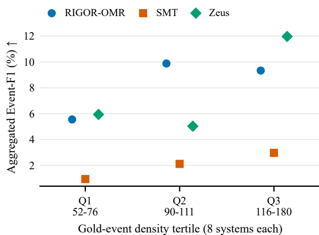
Figure A3: Exploratory Debussy density stratification. Points show aggregated Event-F1 within predeclared gold-event tertiles of eight systems each. No confidence intervals are shown because tertile-level intervals were not estimated; the non-monotonic pattern is descriptive rather than confirmatory.
