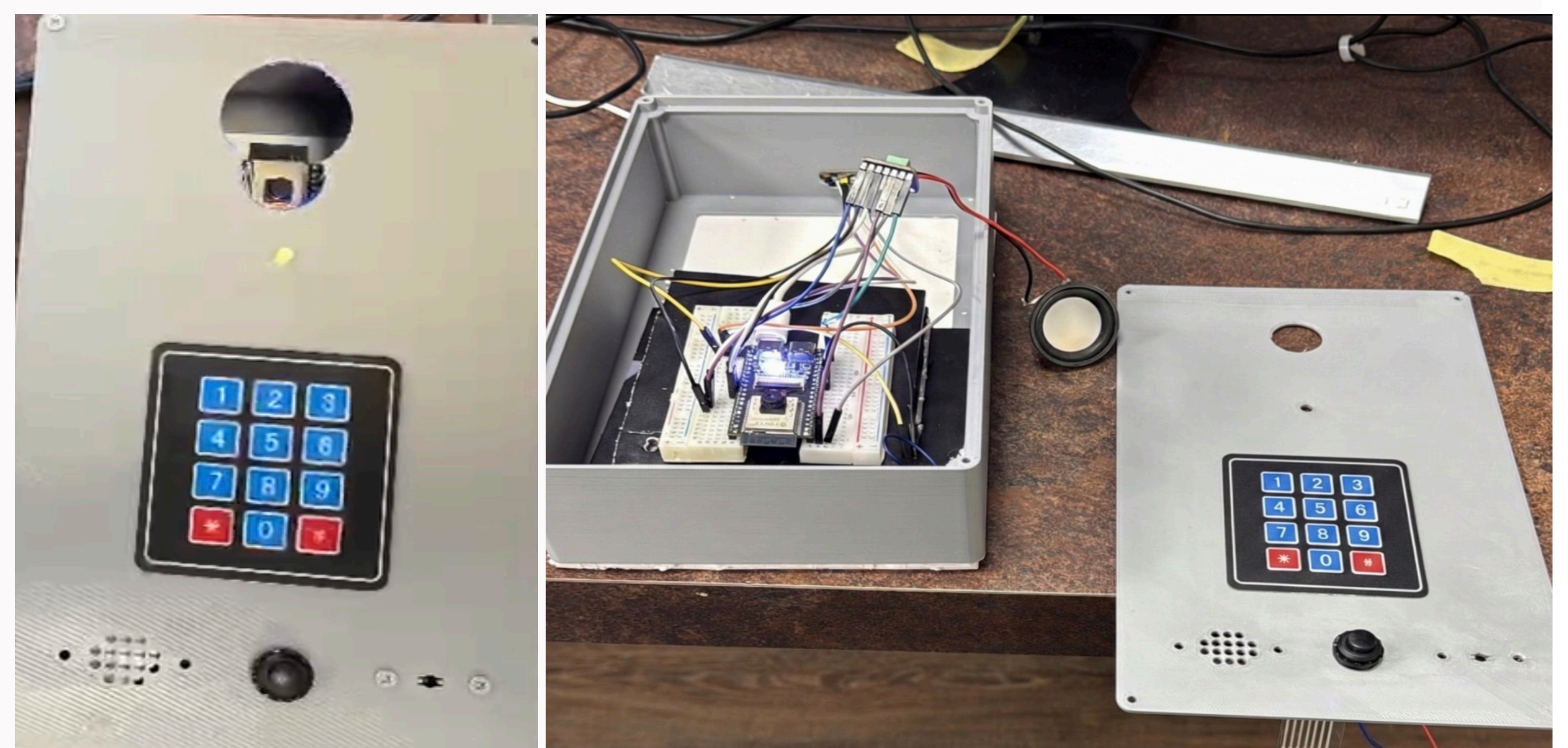
Physical Prototype
