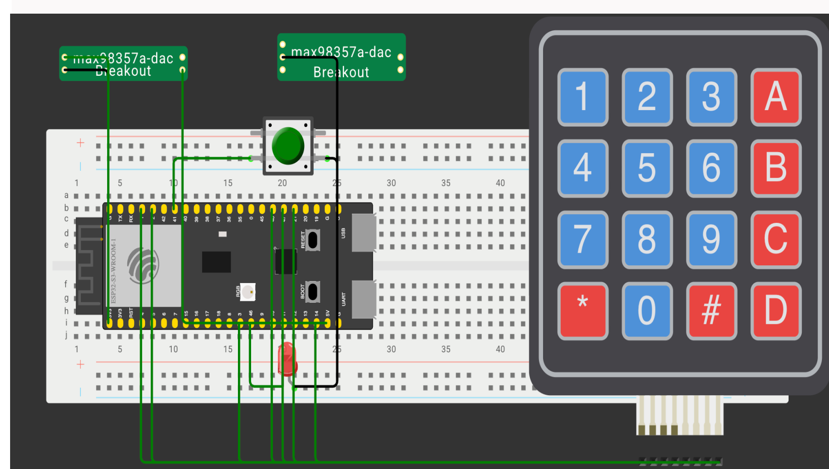
Wiring Digram
