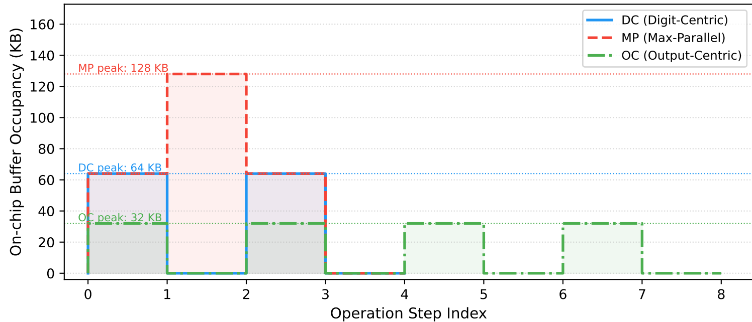
Fig. 5-2 Dynamic Memory Trace: DC vs MP vs OC ( N = 4096 , sizeP = 2, 2 digits)
