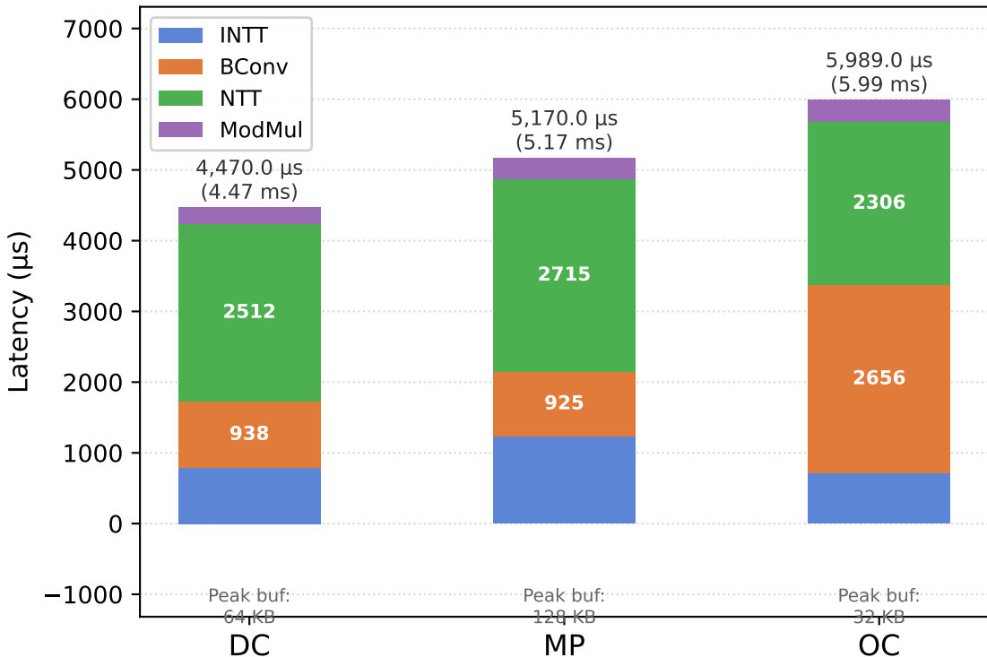
Fig. 5-3 Latency Breakdown by Scheduling Strategy ( N = 4096 , sizeP = 2, 2 digits, CPU software path)
