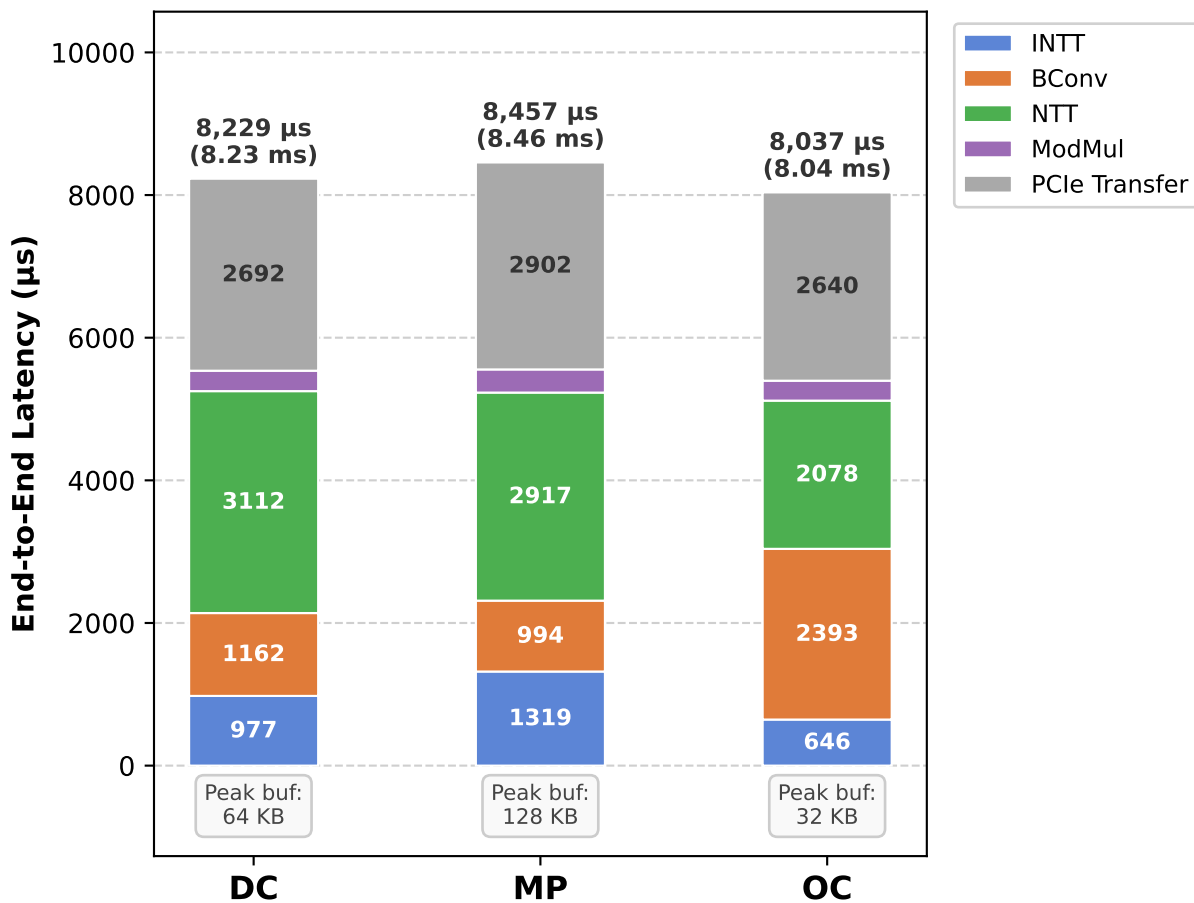
Fig. 5-3 End-to-End Latency Breakdown by Scheduling Strategy ( N = 4096 , sizeP = 2, 2 digits, FPGA Offload)
