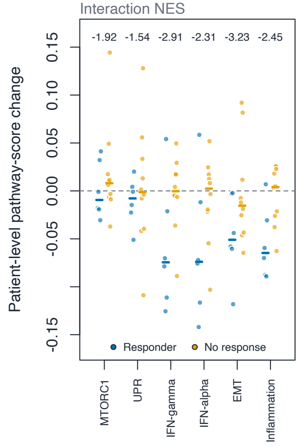
F Patient score changes
