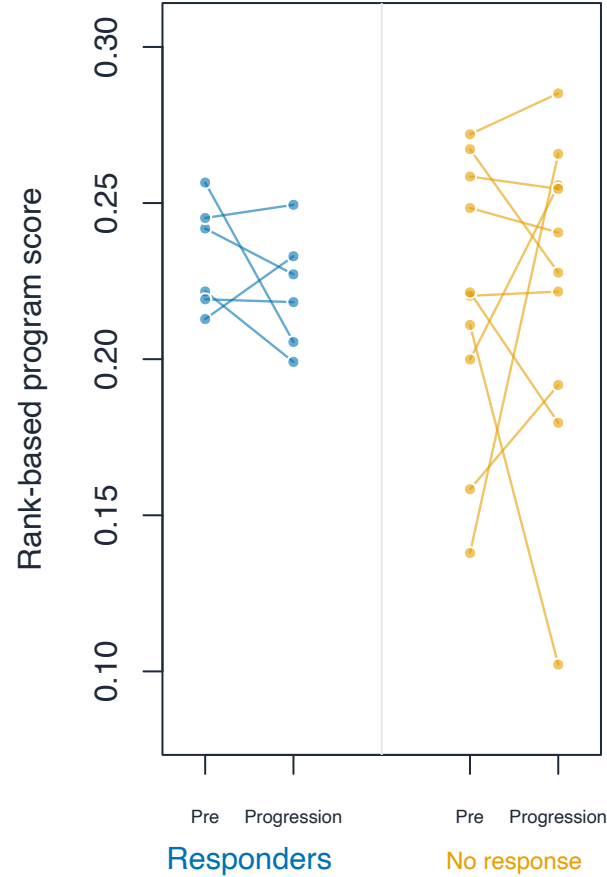
C Unfolded protein response
