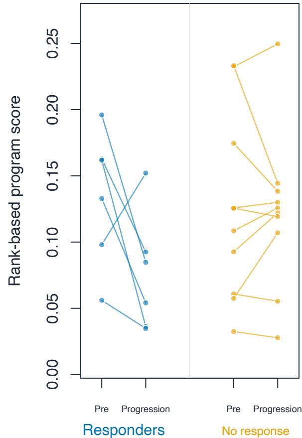
E IFN-gamma response
