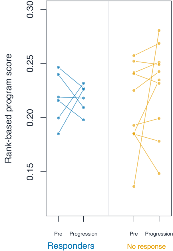
B MTORC1 signaling
