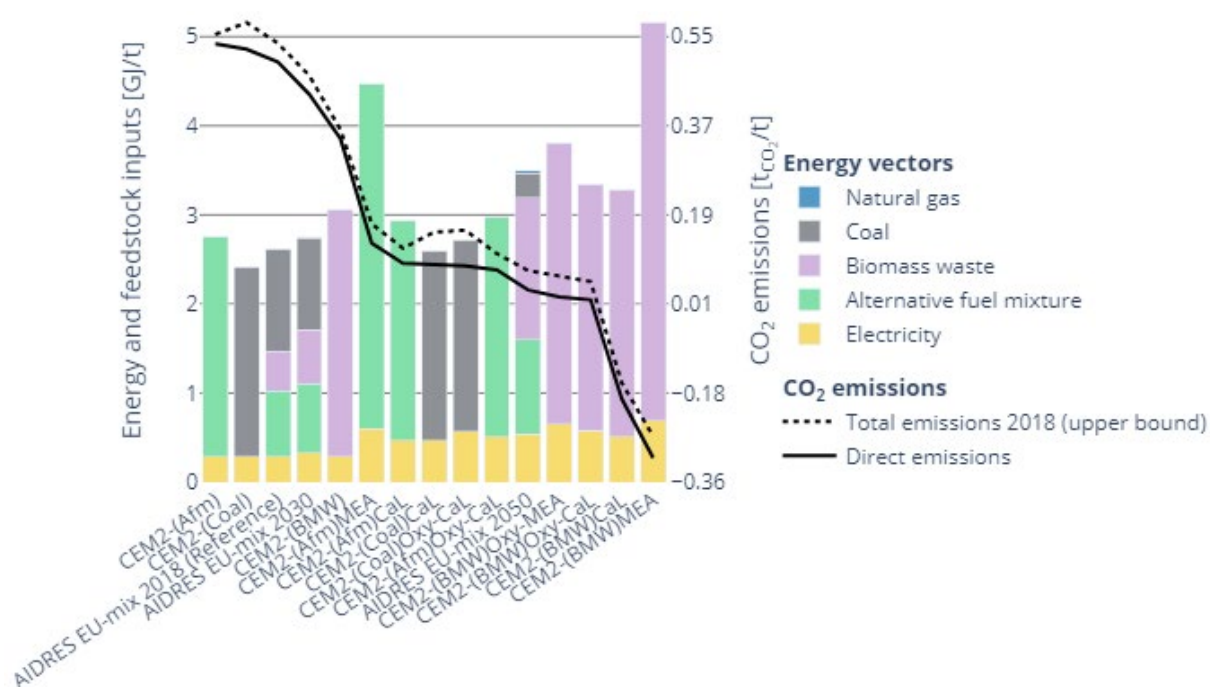
Figure 22: Energy and feedstock flows [GJ/t] and emissions [tCO 2 /t] for Portland cement II production routes.
