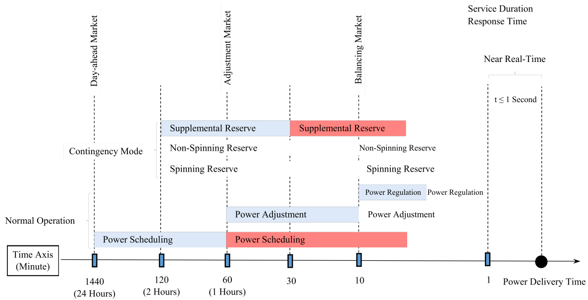
Fig. 8. Time response and duration of short-term market floors and ancillary services in a graphical presentation.
