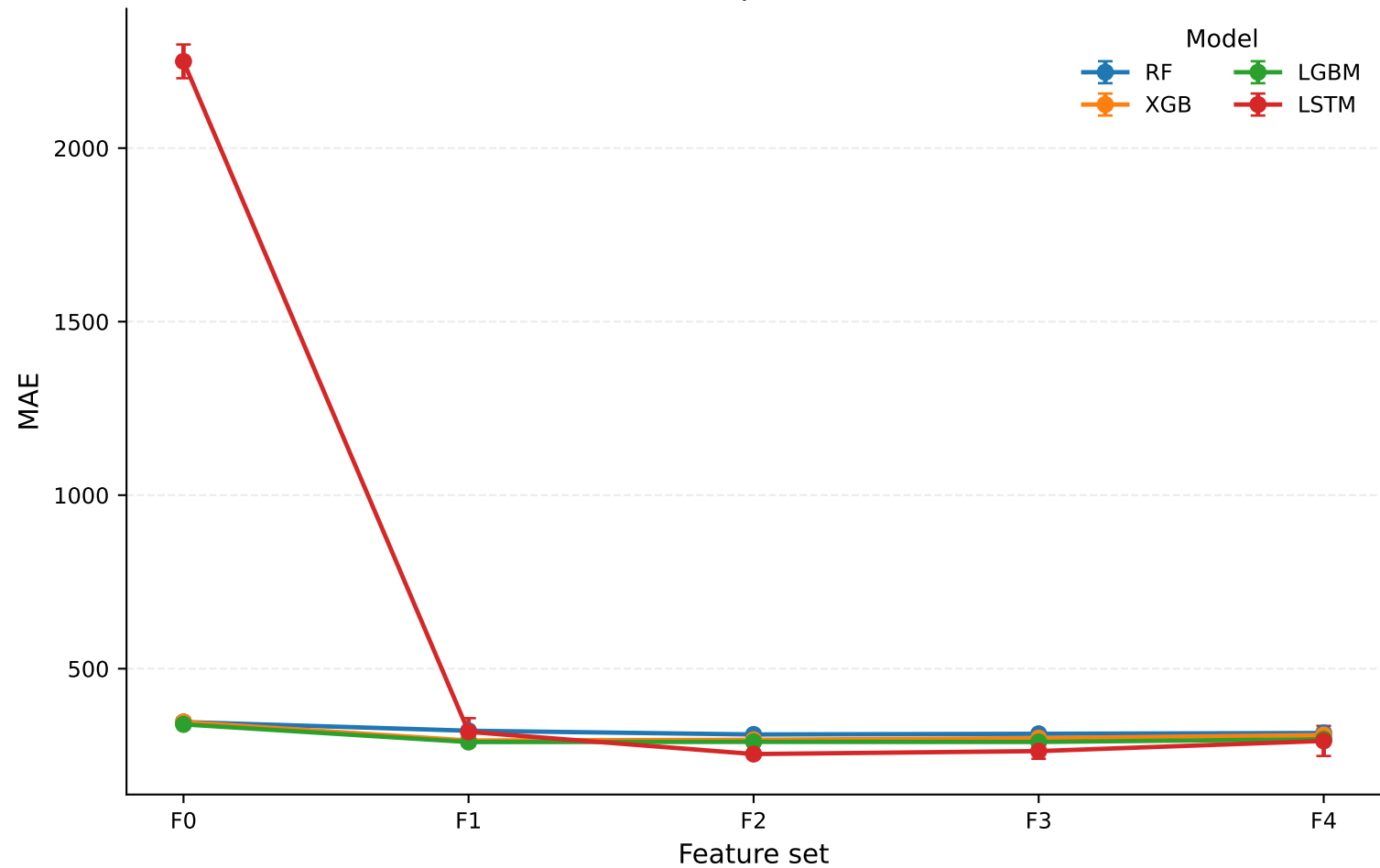
MAE across temporal feature sets
