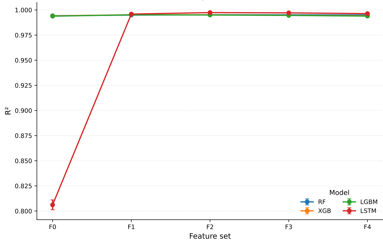
R 2 across temporal feature sets
