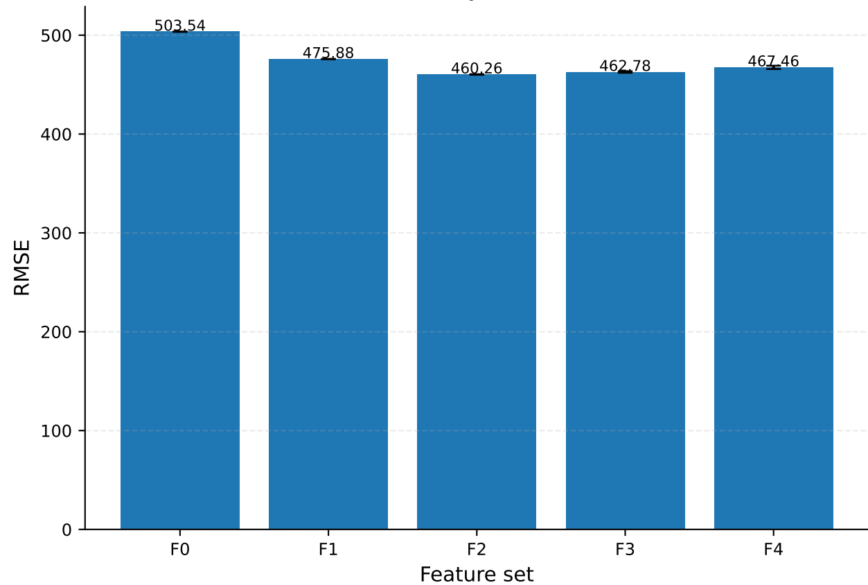
RF: RMSE by feature set
