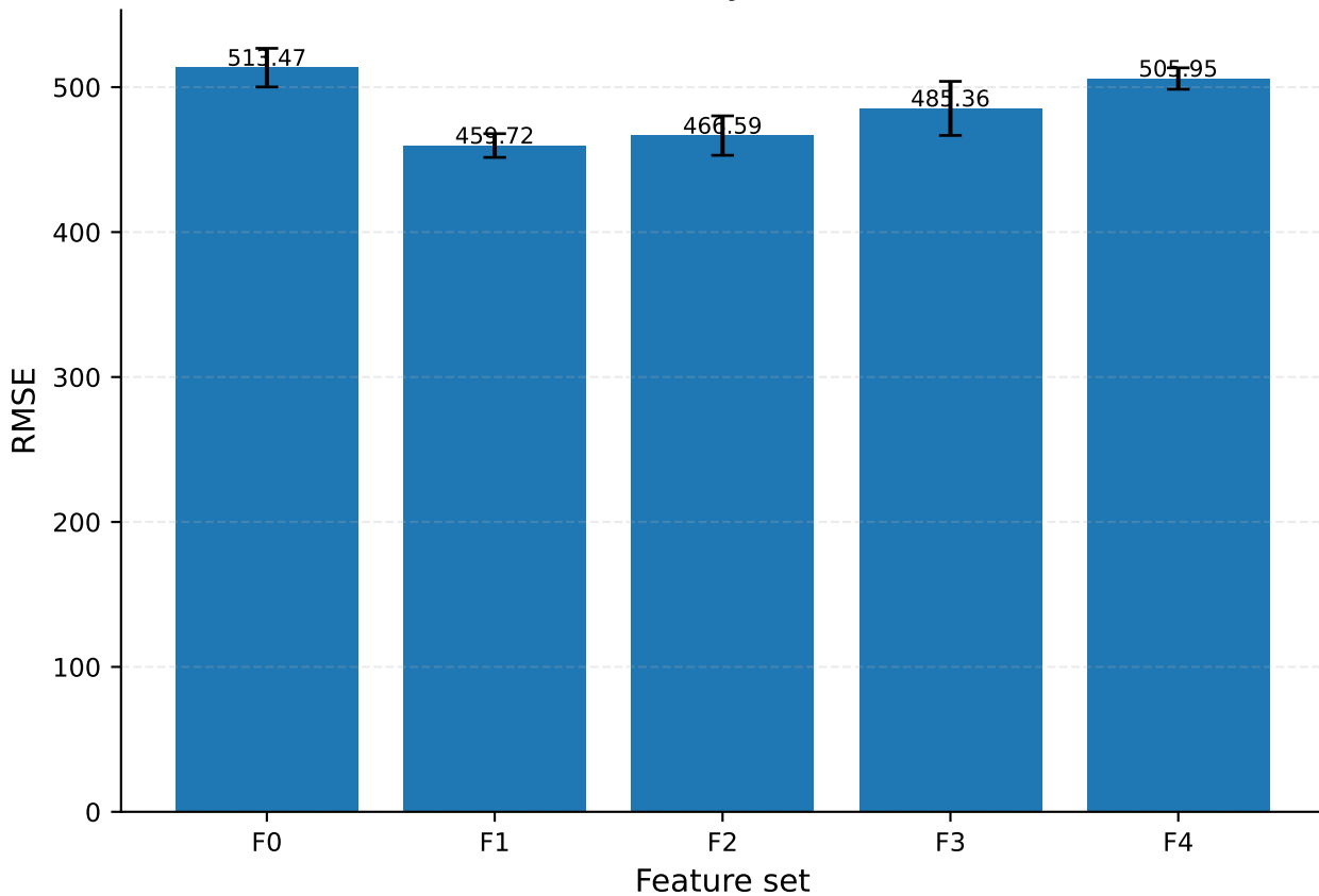
XGB: RMSE by feature set
