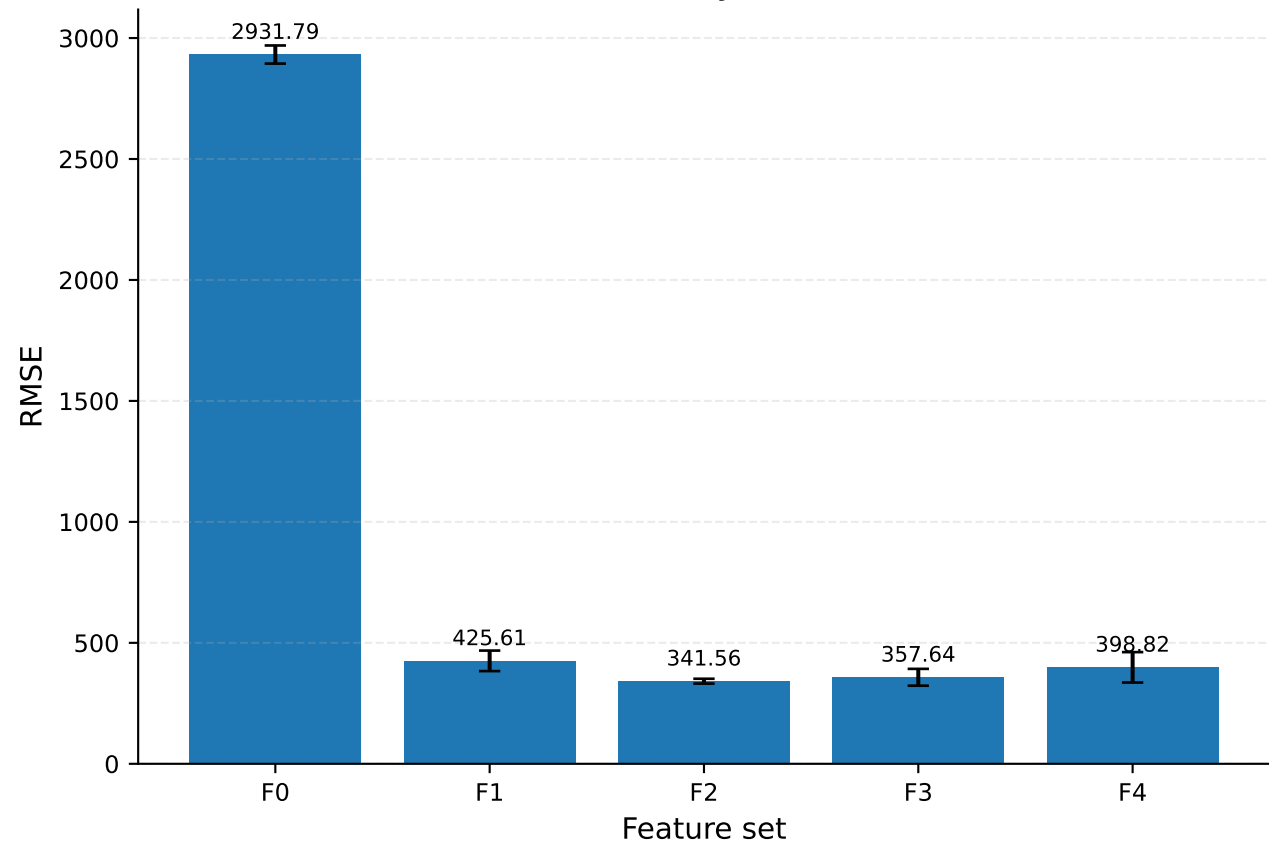
LSTM: RMSE by feature set
