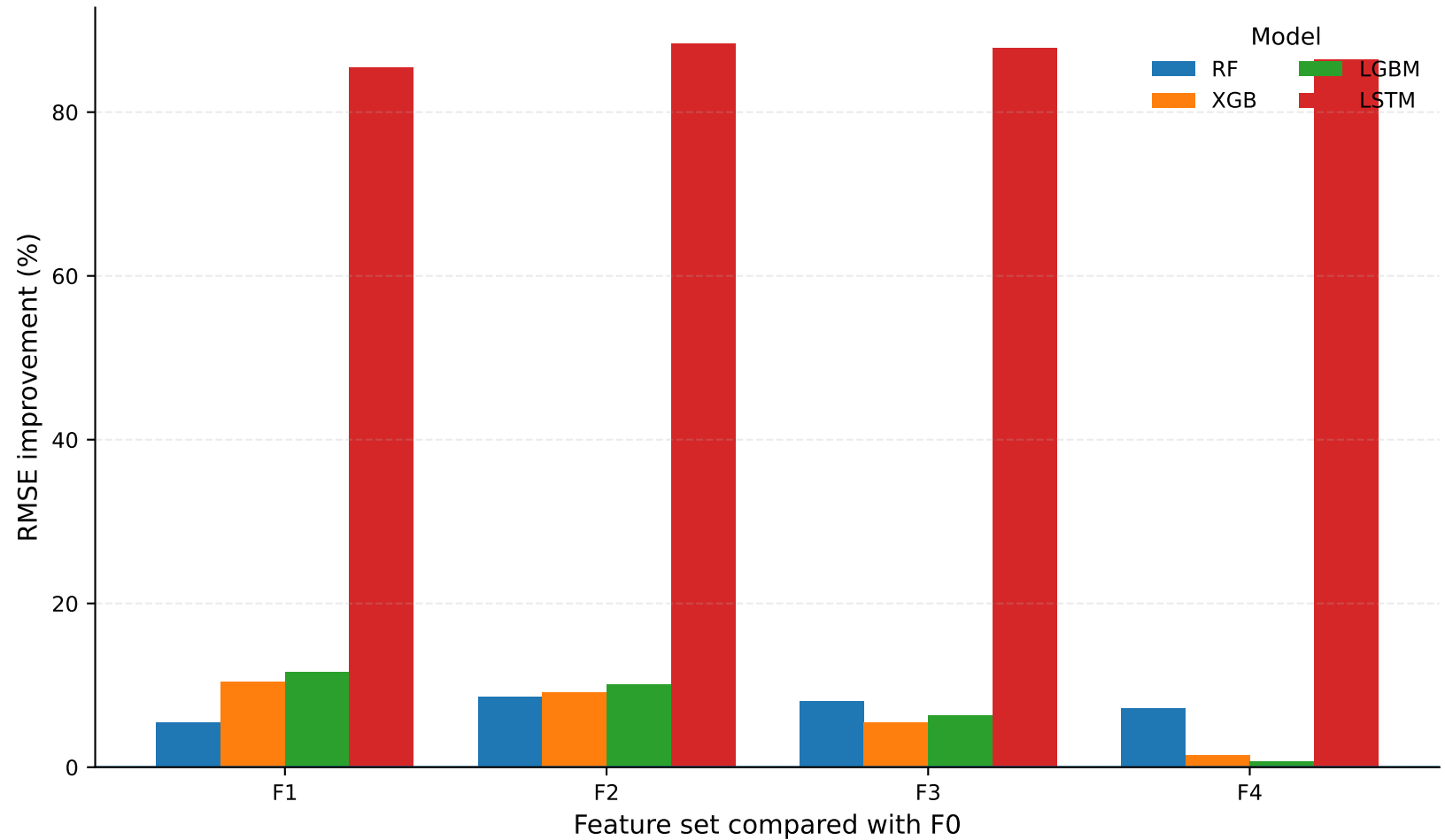
RMSE improvement relative to F0
