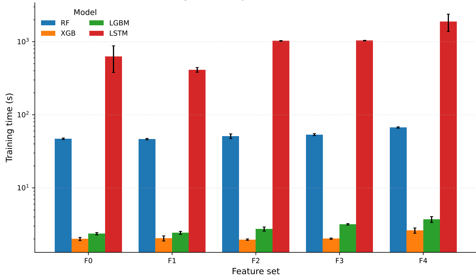
Training time (s) by model and feature set
